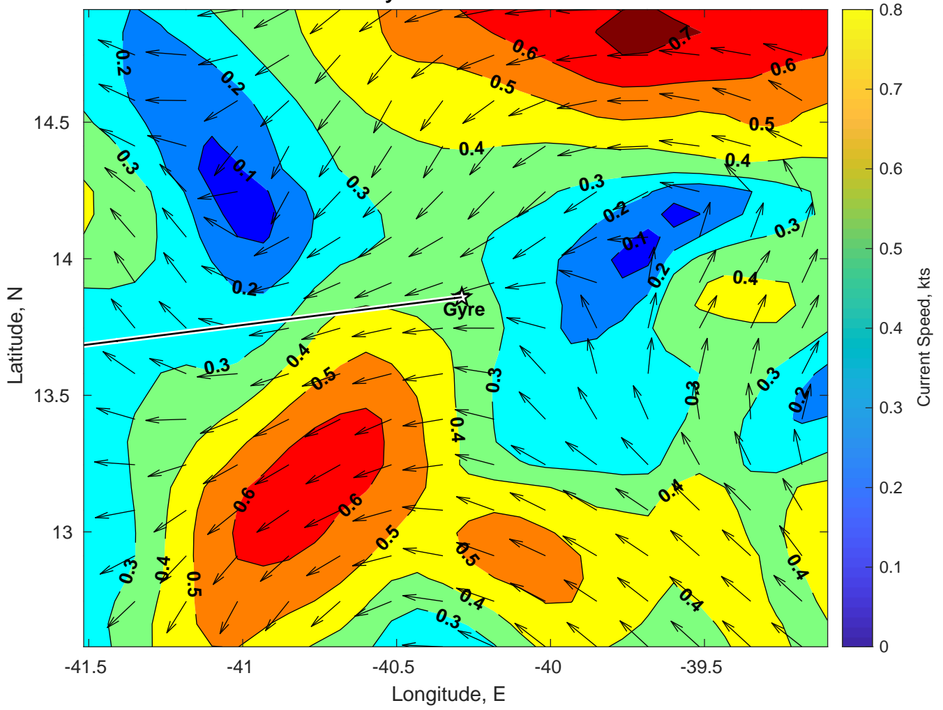
Surface Currents for Gyre at 20-Jan-2025 00:00:00
