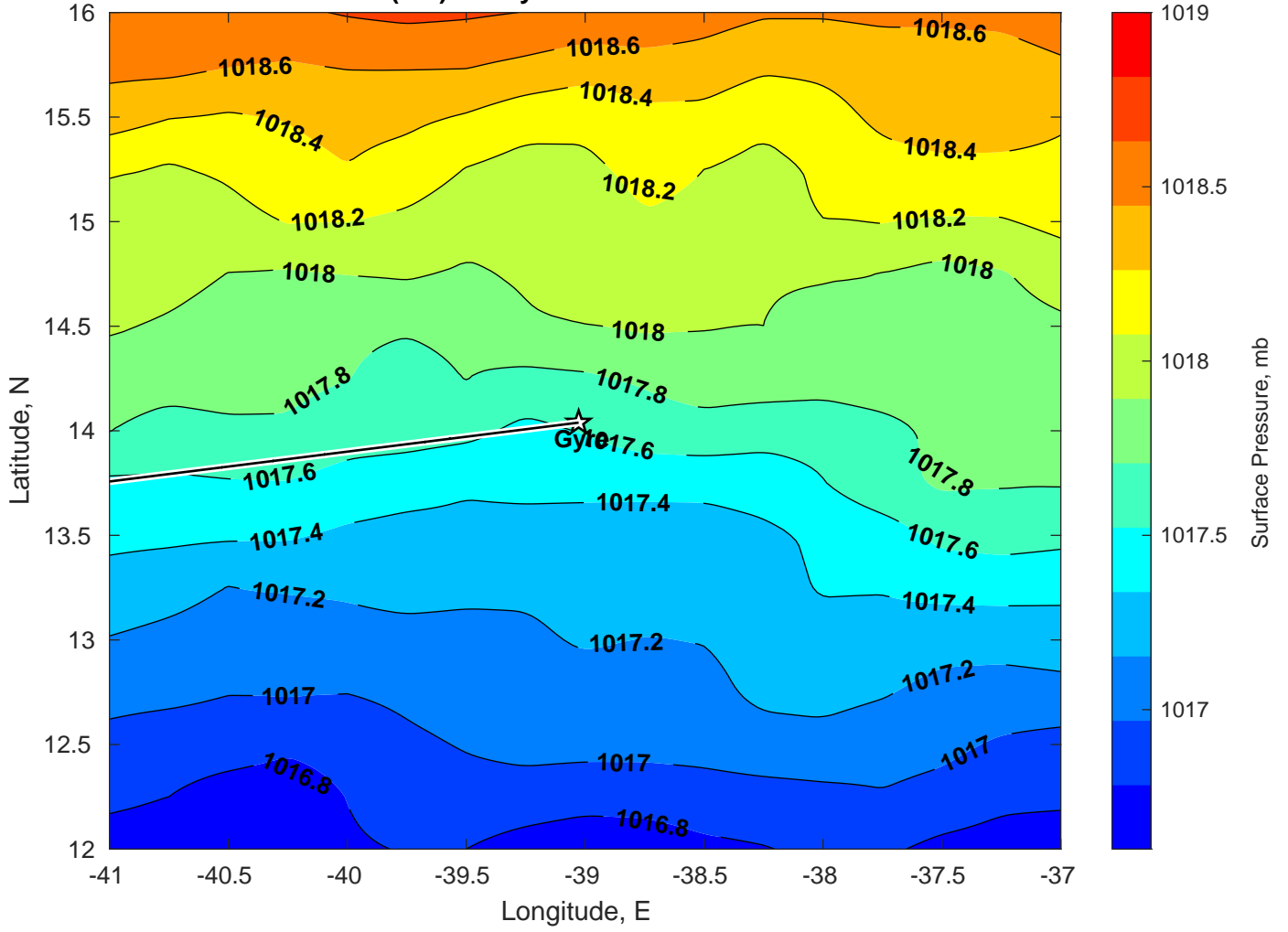
Surface Pressure (mb) for Gyre at 21-Jan-2025 00:00:00
