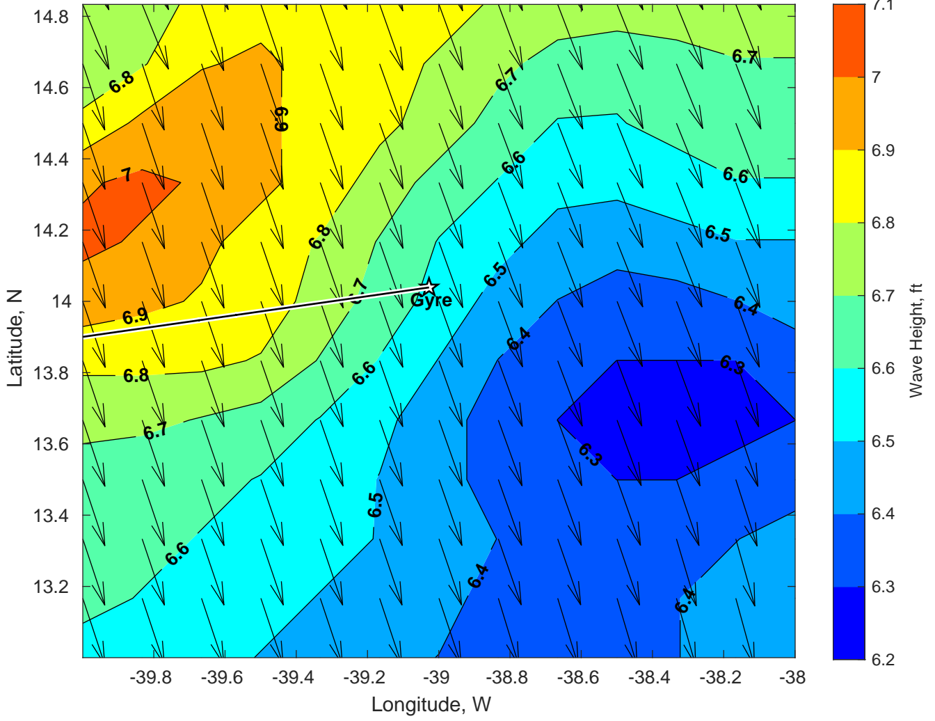
Wave Height (ft) for Gyre at 21-Jan-2025 09:00:00
