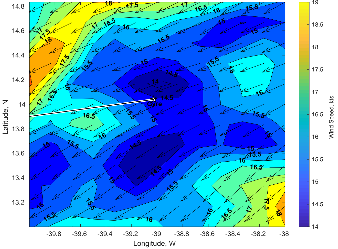
Winds (kts) for Gyre at 21-Jan-2025 09:00:00
