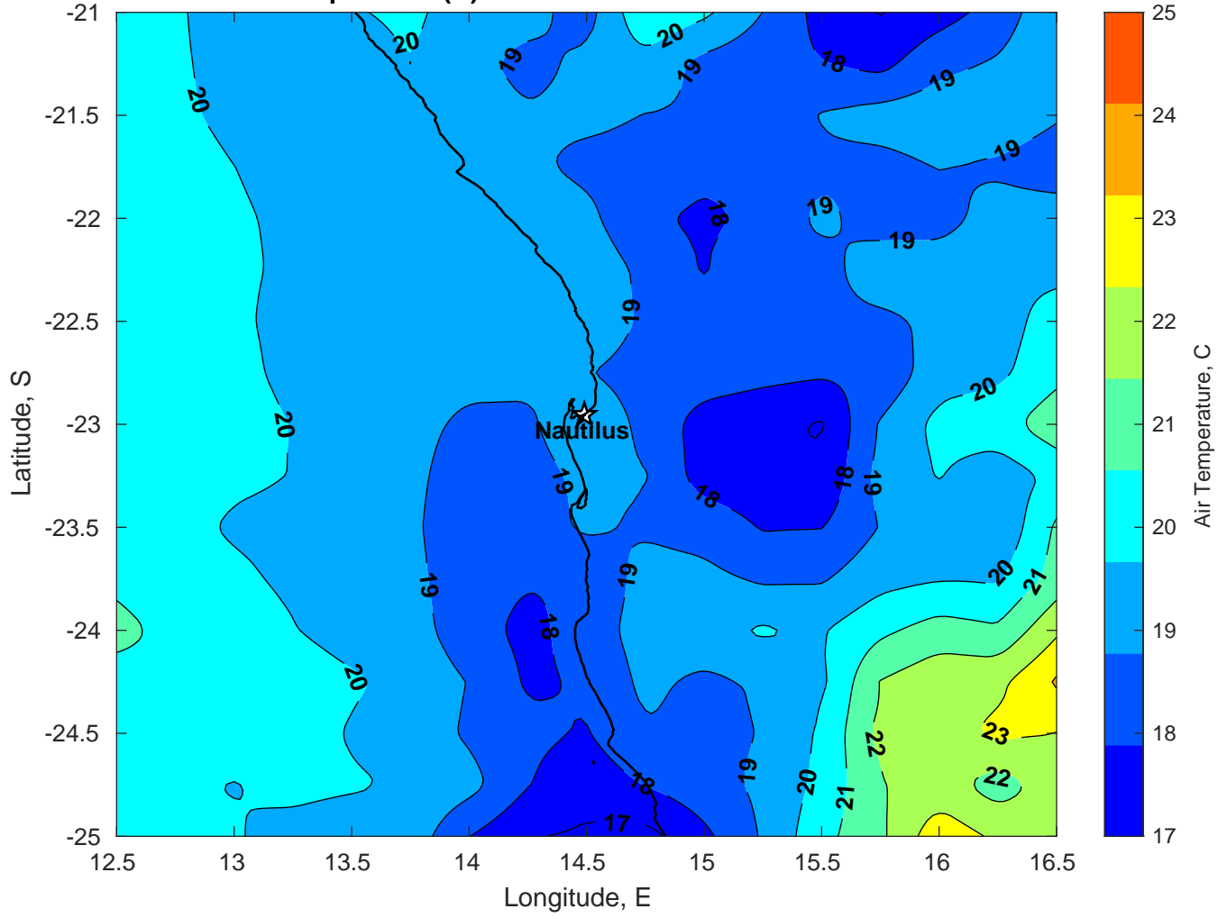
Air Temperature (C) for Nautilus at 21-Jan-2025
