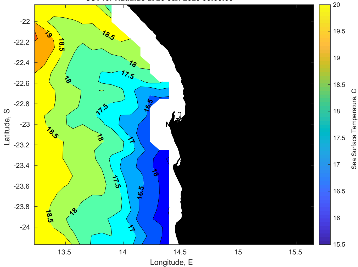
SST for Nautilus at 20-Jan-2025 00:00:00
