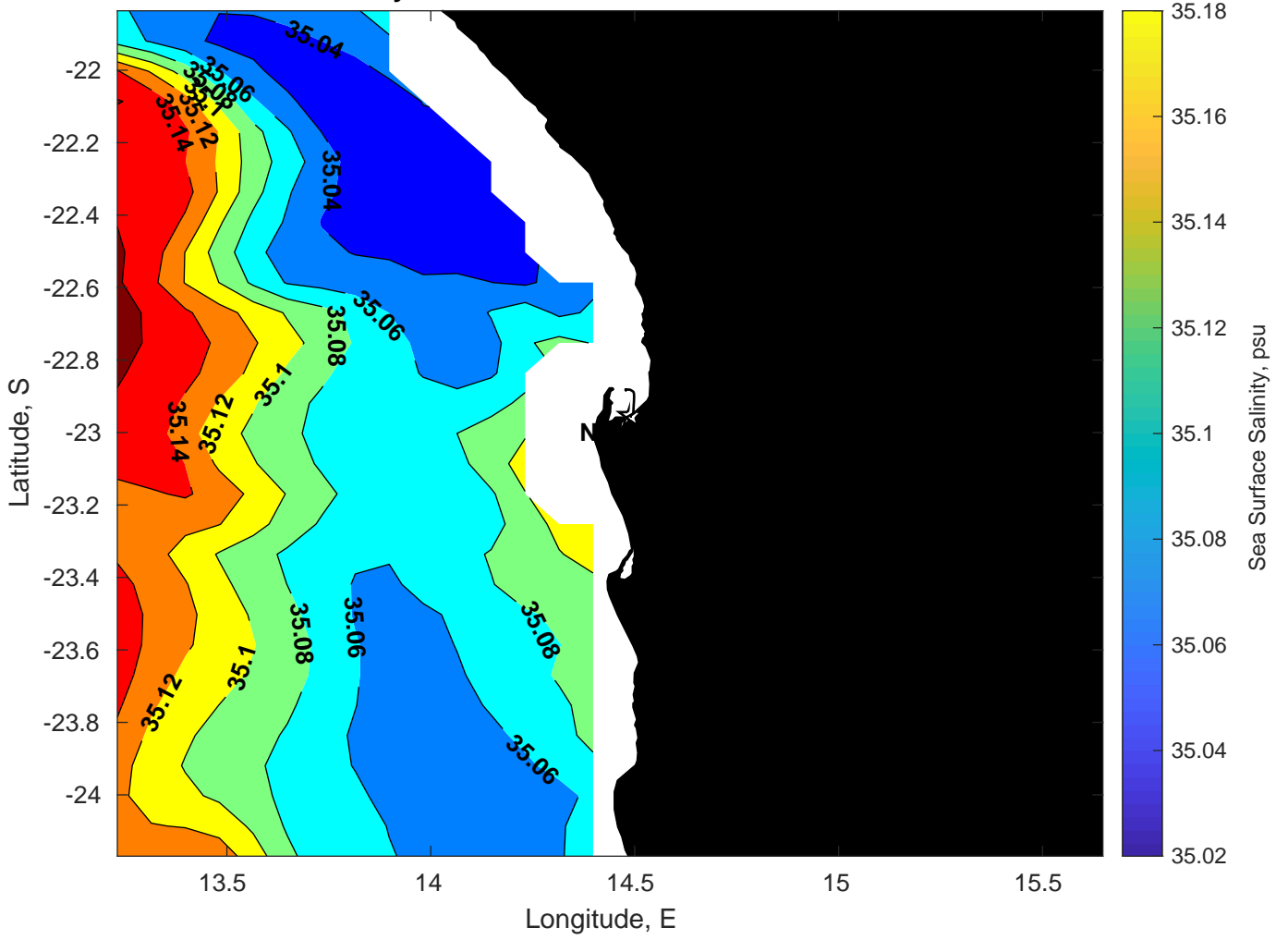
Surface Salinity for Nautilus at 20-Jan-2025 00:00:00
