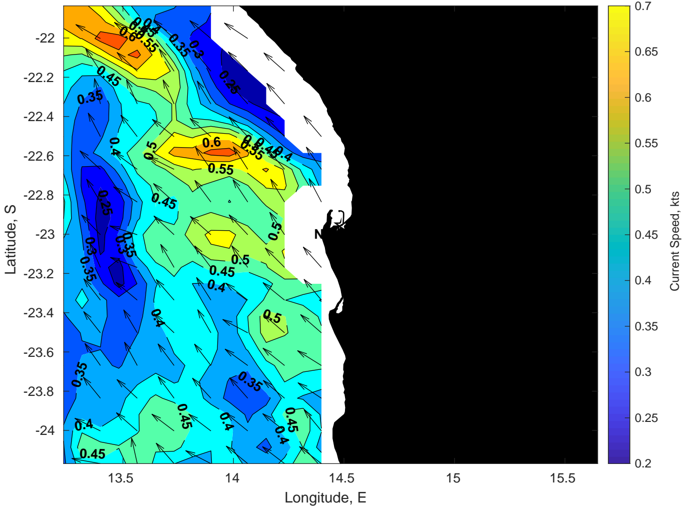
Surface Currents for Nautilus at 20-Jan-2025 00:00:00
