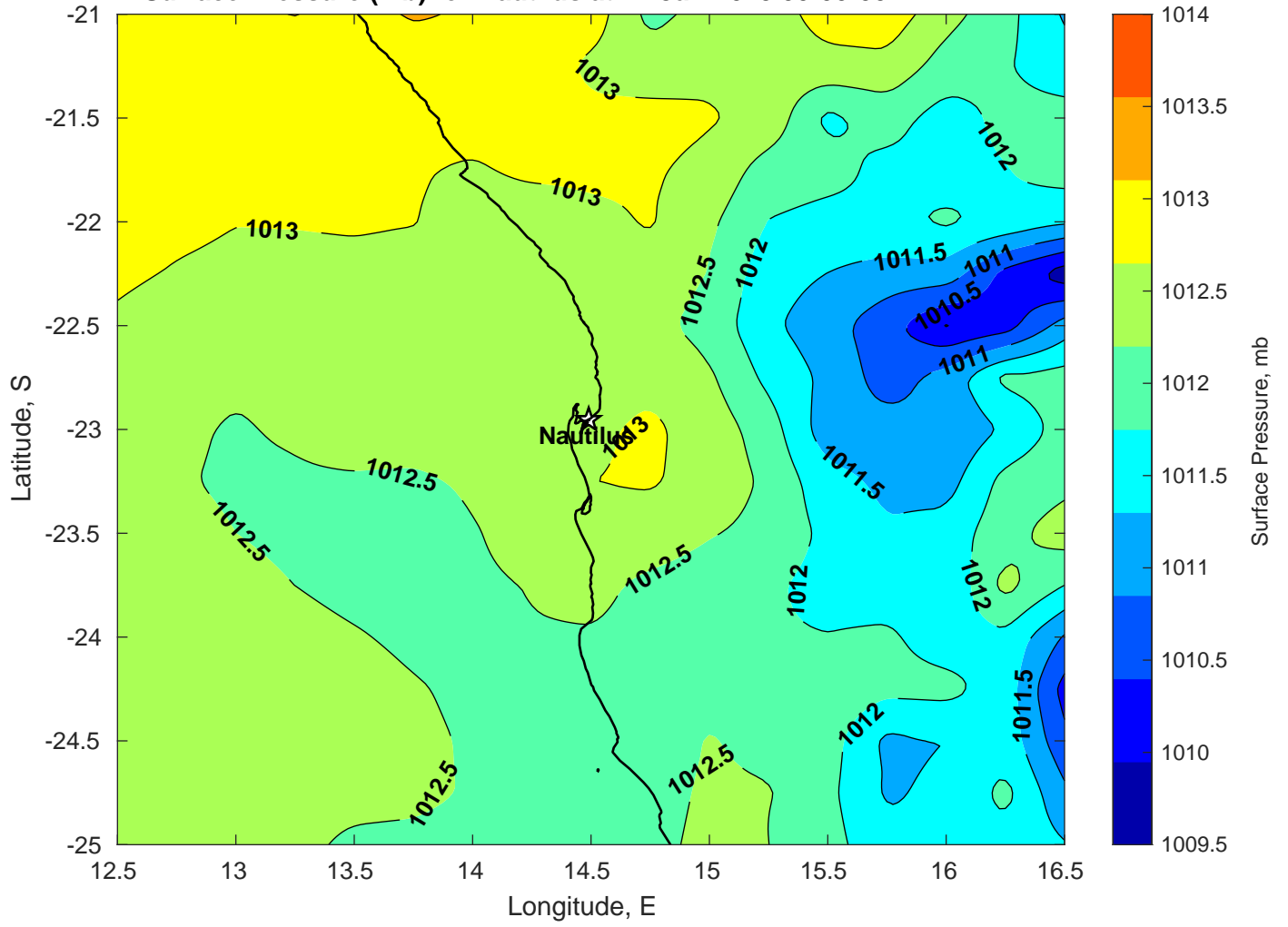
Surface Pressure (mb) for Nautilus at 22-Jan-2025 00:00:00
