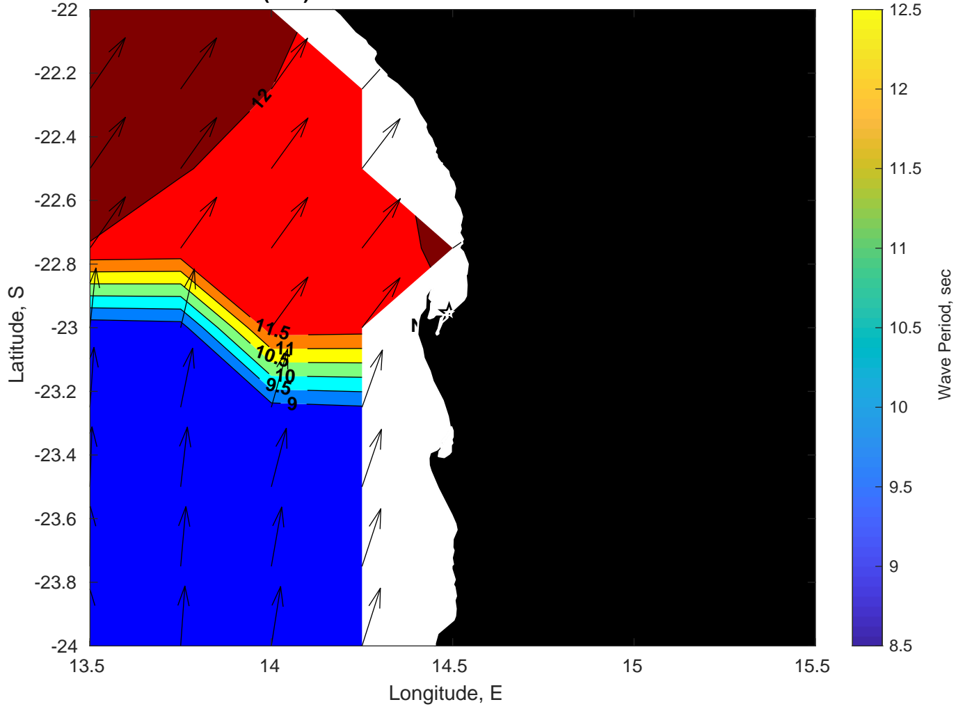
Wave Period (sec) for Nautilus at 21-Jan-2025 09:00:00
