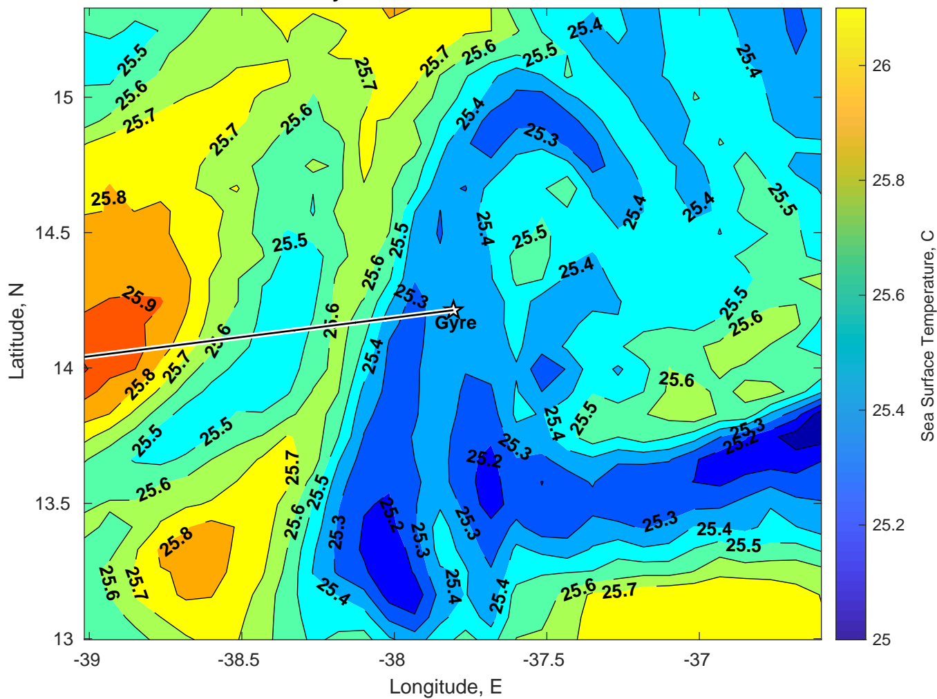
SST for Gyre at 21-Jan-2025 00:00:00
