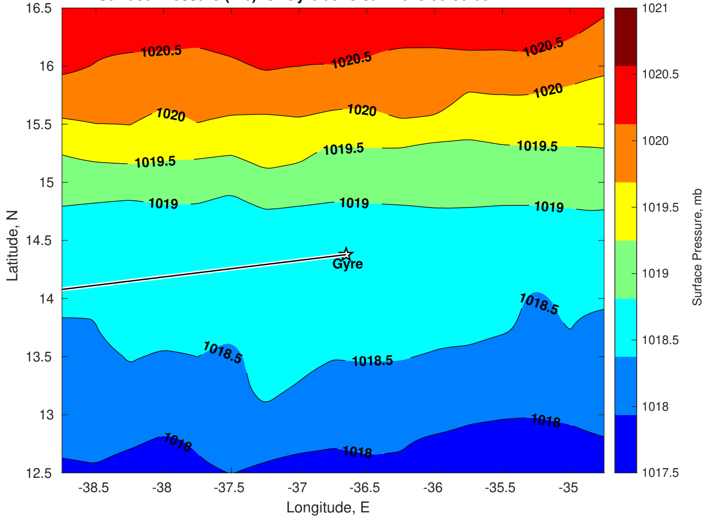
Surface Pressure (mb) for Gyre at 23-Jan-2025 00:00:00
