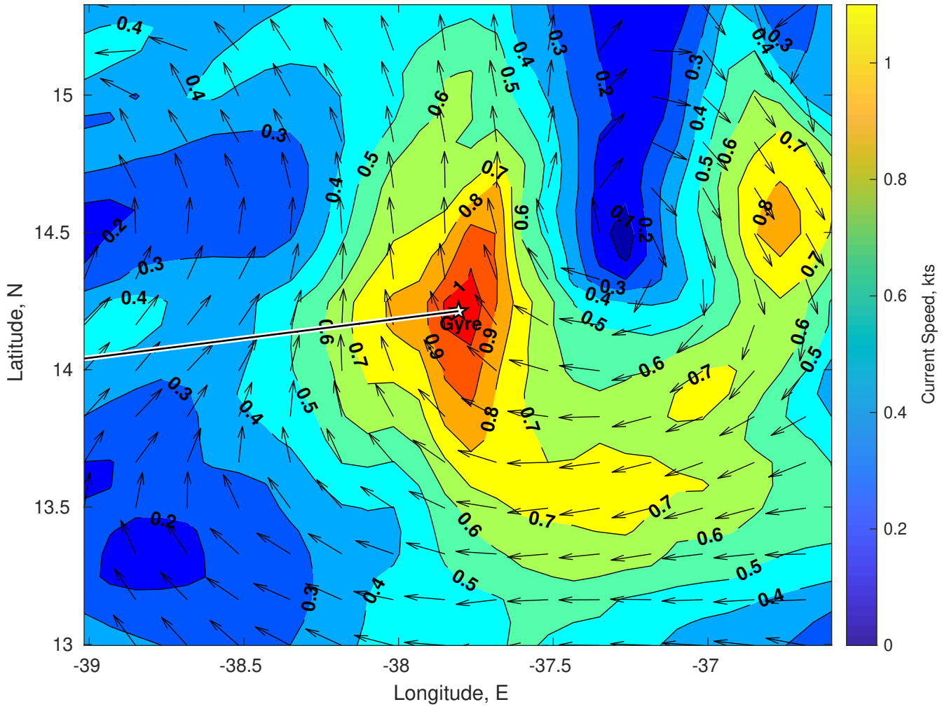
Surface Currents for Gyre at 21-Jan-2025 00:00:00
