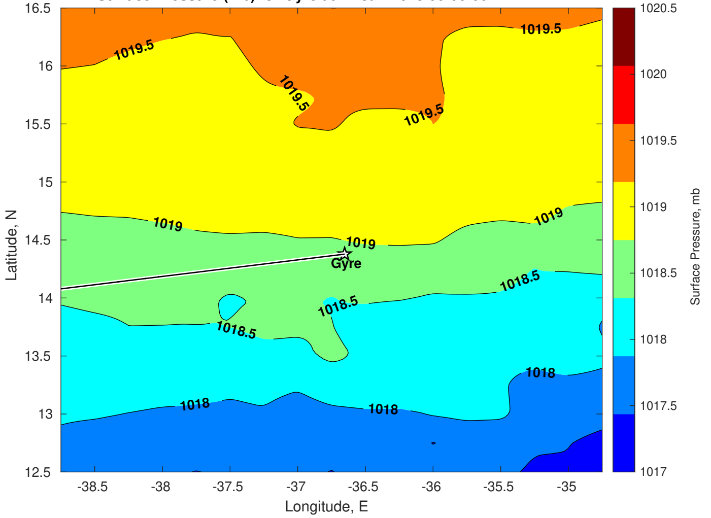
Surface Pressure (mb) for Gyre at 24-Jan-2025 00:00:00
