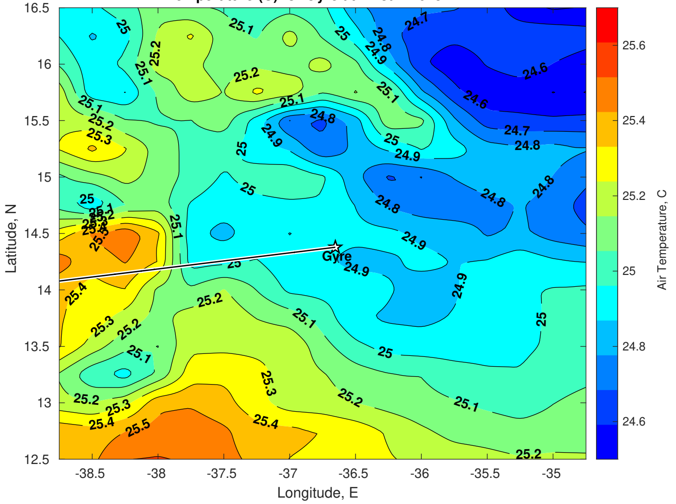
Air Temperature (C) for Gyre at 22-Jan-2025
