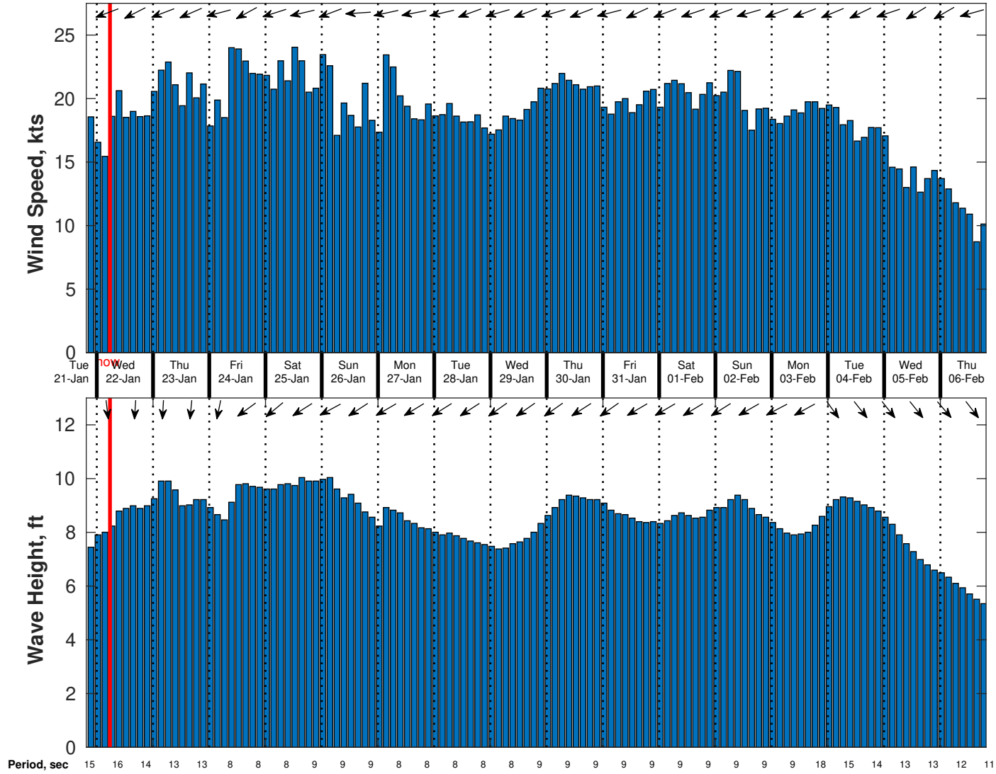
Wind & Wave Forecast for Gyre from 21-Jan-2025 20:00:00 to 06-Feb-2025 20:00:00
