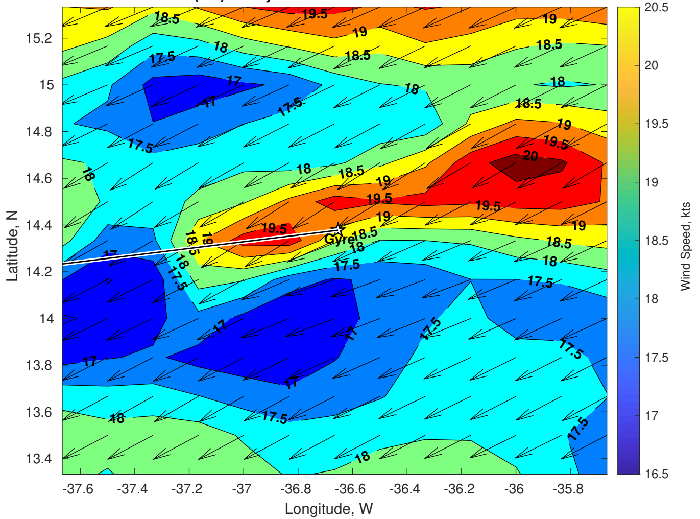
Winds (kts) for Gyre at 22-Jan-2025 09:00:00
