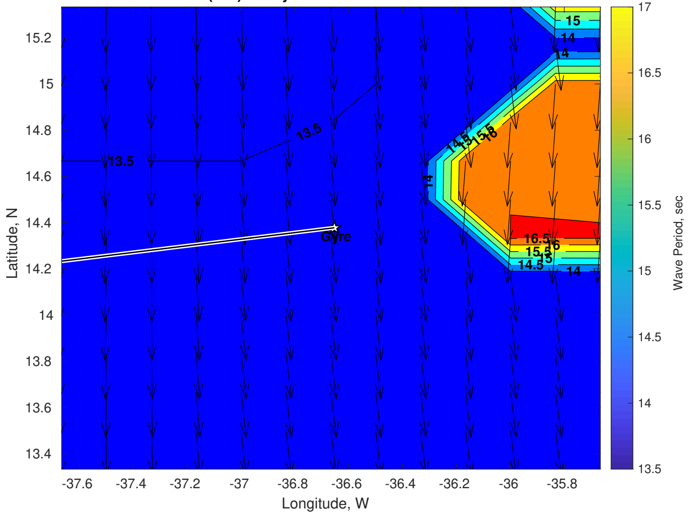
Wave Period (sec) for Gyre at 22-Jan-2025 09:00:00
