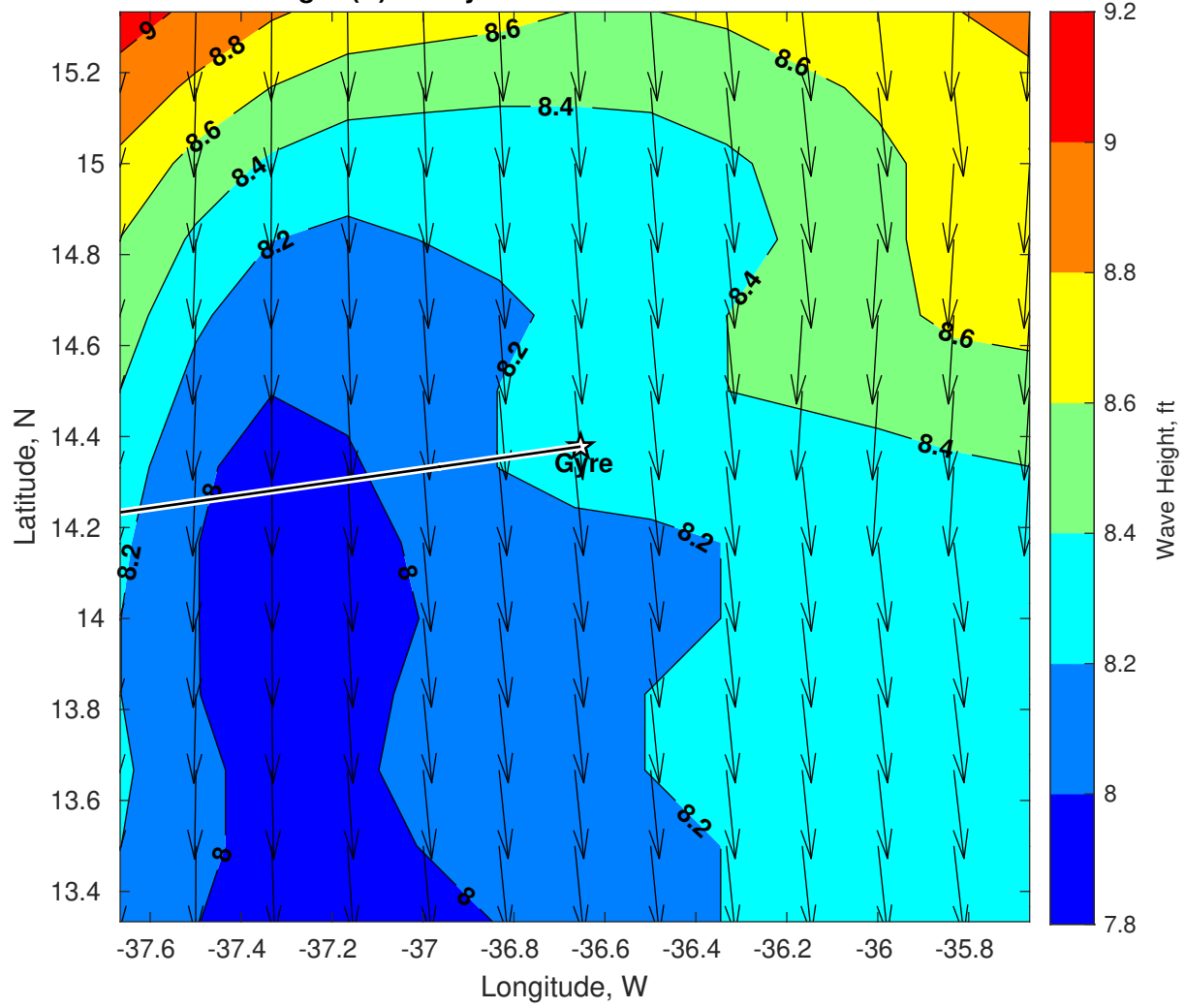
Wave Height (ft) for Gyre at 22-Jan-2025 09:00:00
