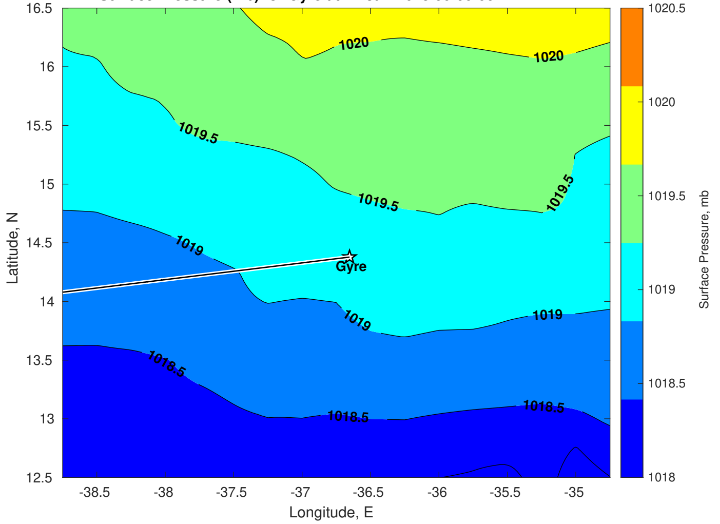
Surface Pressure (mb) for Gyre at 22-Jan-2025 00:00:00
