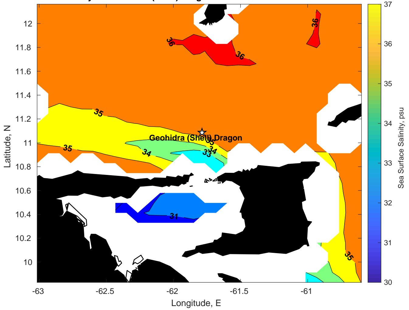
Surface Salinity for Geohidra (Shell) Dragon at 22-Jan-2025 00:00:00
