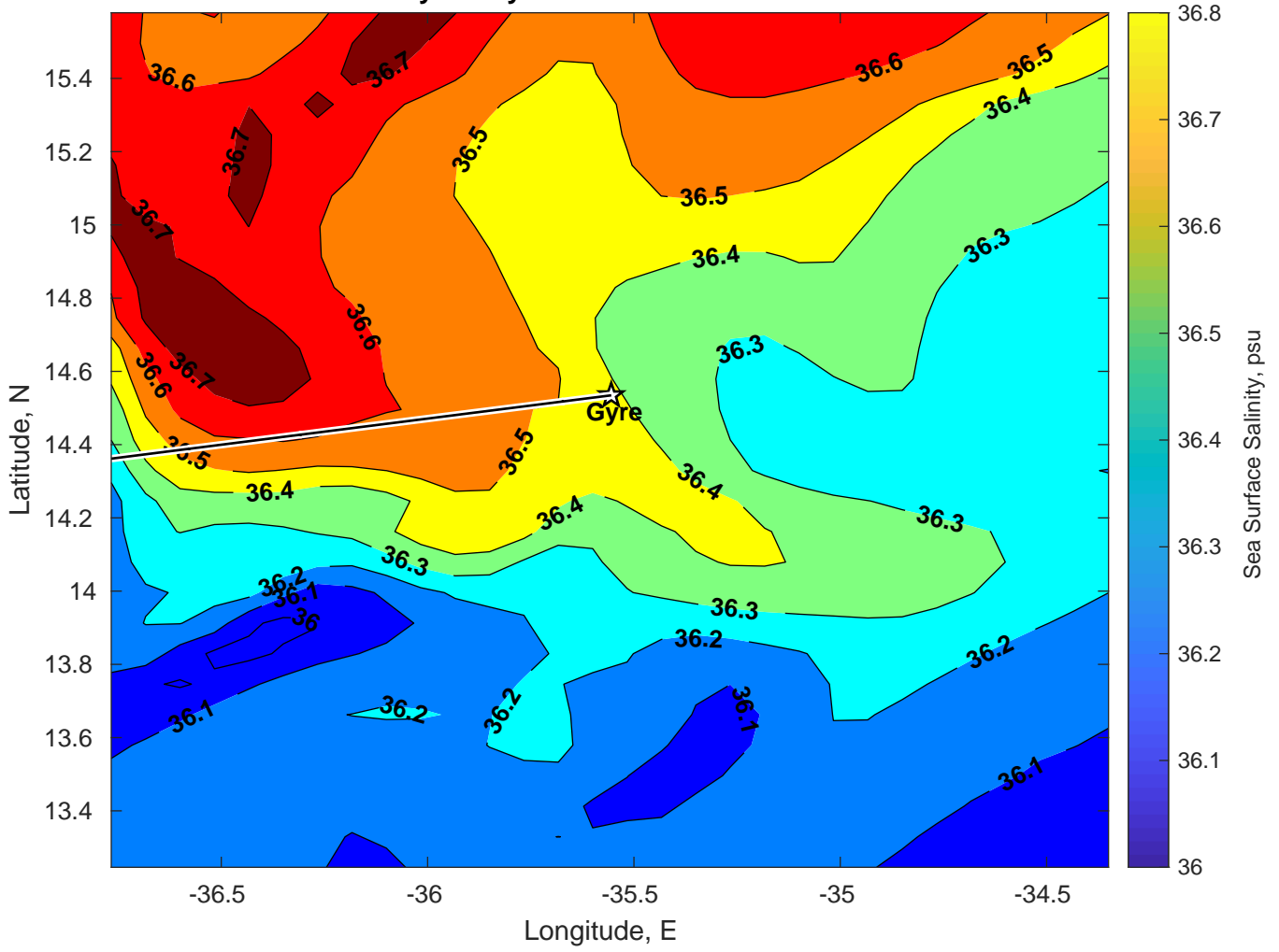
Surface Salinity for Gyre at 22-Jan-2025 00:00:00
