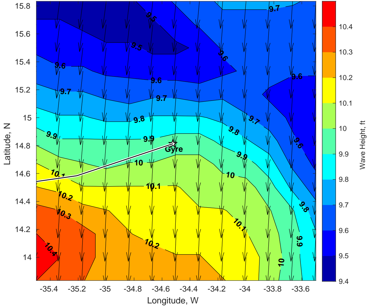
Wave Height (ft) for Gyre at 23-Jan-2025 09:00:00
