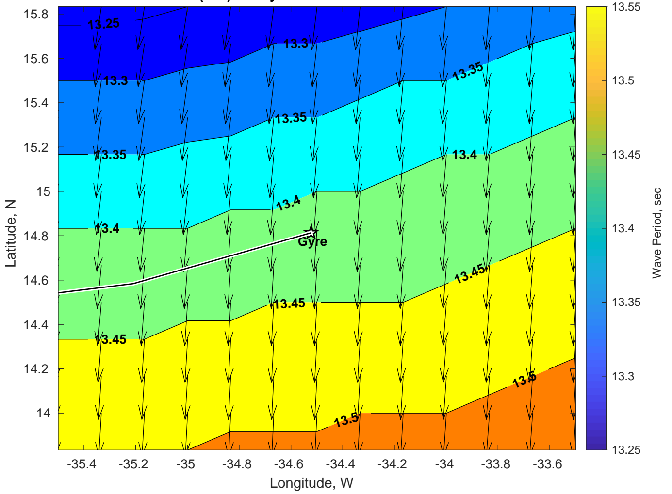
Wave Period (sec) for Gyre at 23-Jan-2025 09:00:00
