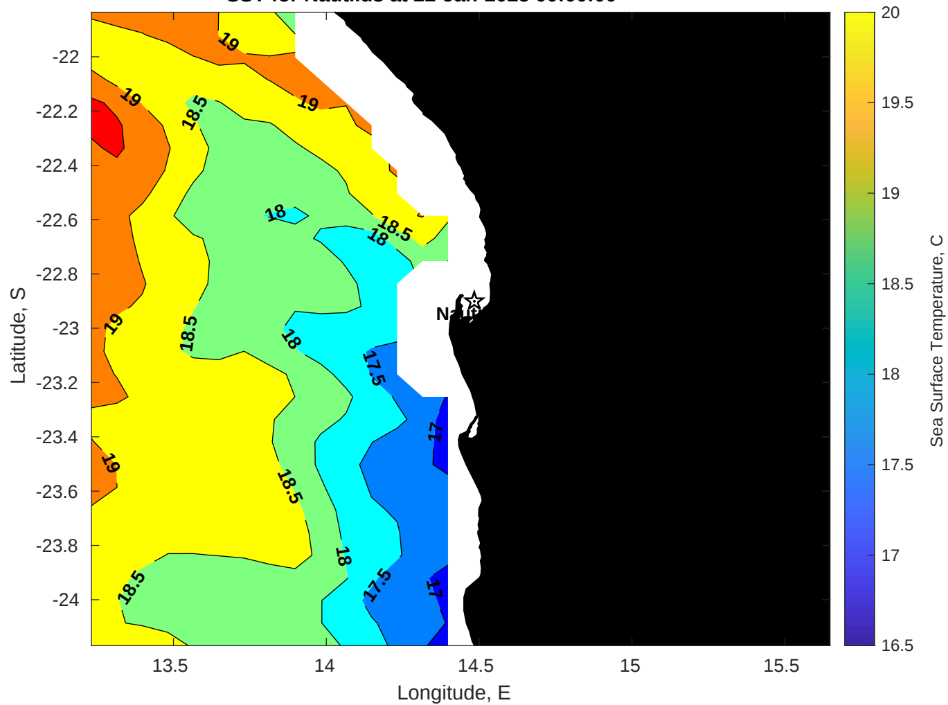
SST for Nautilus at 22-Jan-2025 00:00:00
