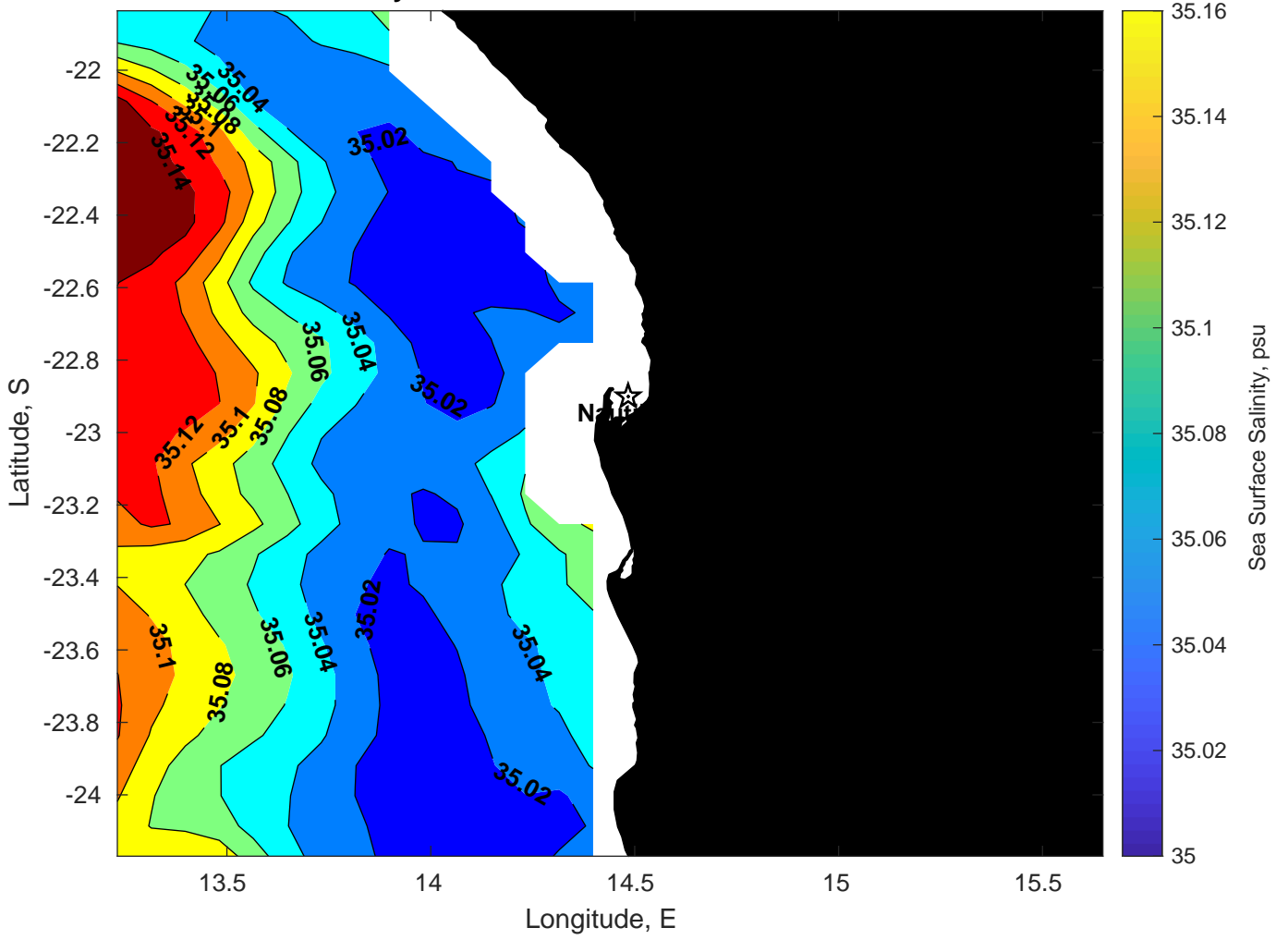
Surface Salinity for Nautilus at 22-Jan-2025 00:00:00
