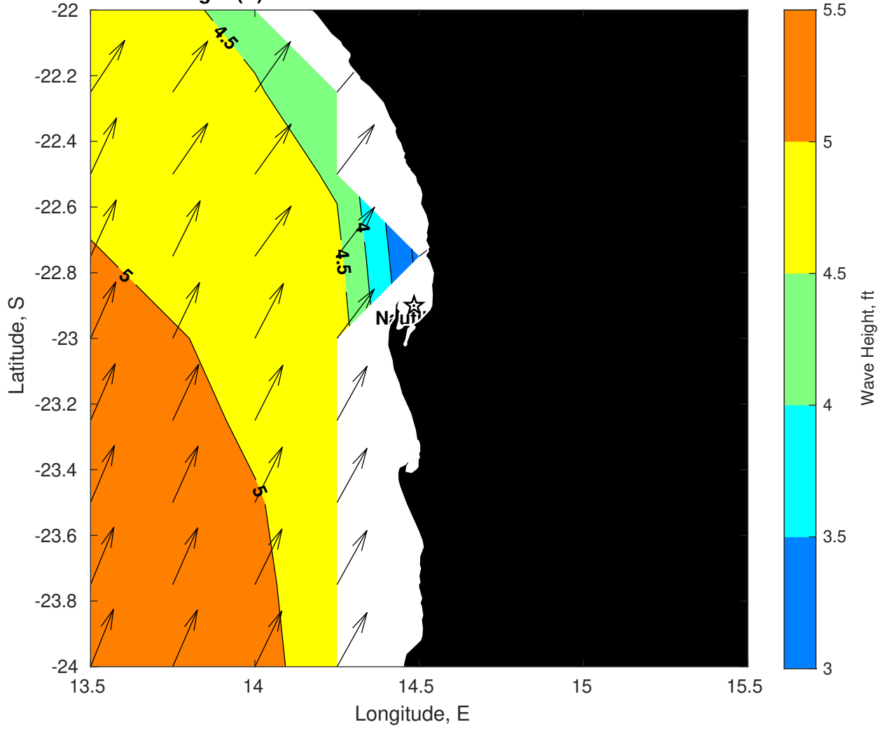
Wave Height (ft) for Nautilus at 23-Jan-2025 09:00:00
