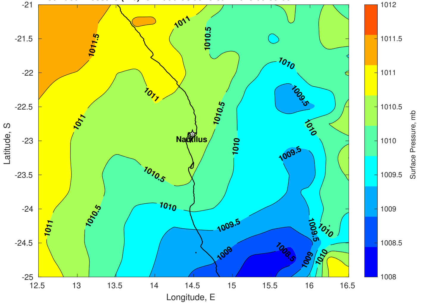
Surface Pressure (mb) for Nautilus at 25-Jan-2025 00:00:00
