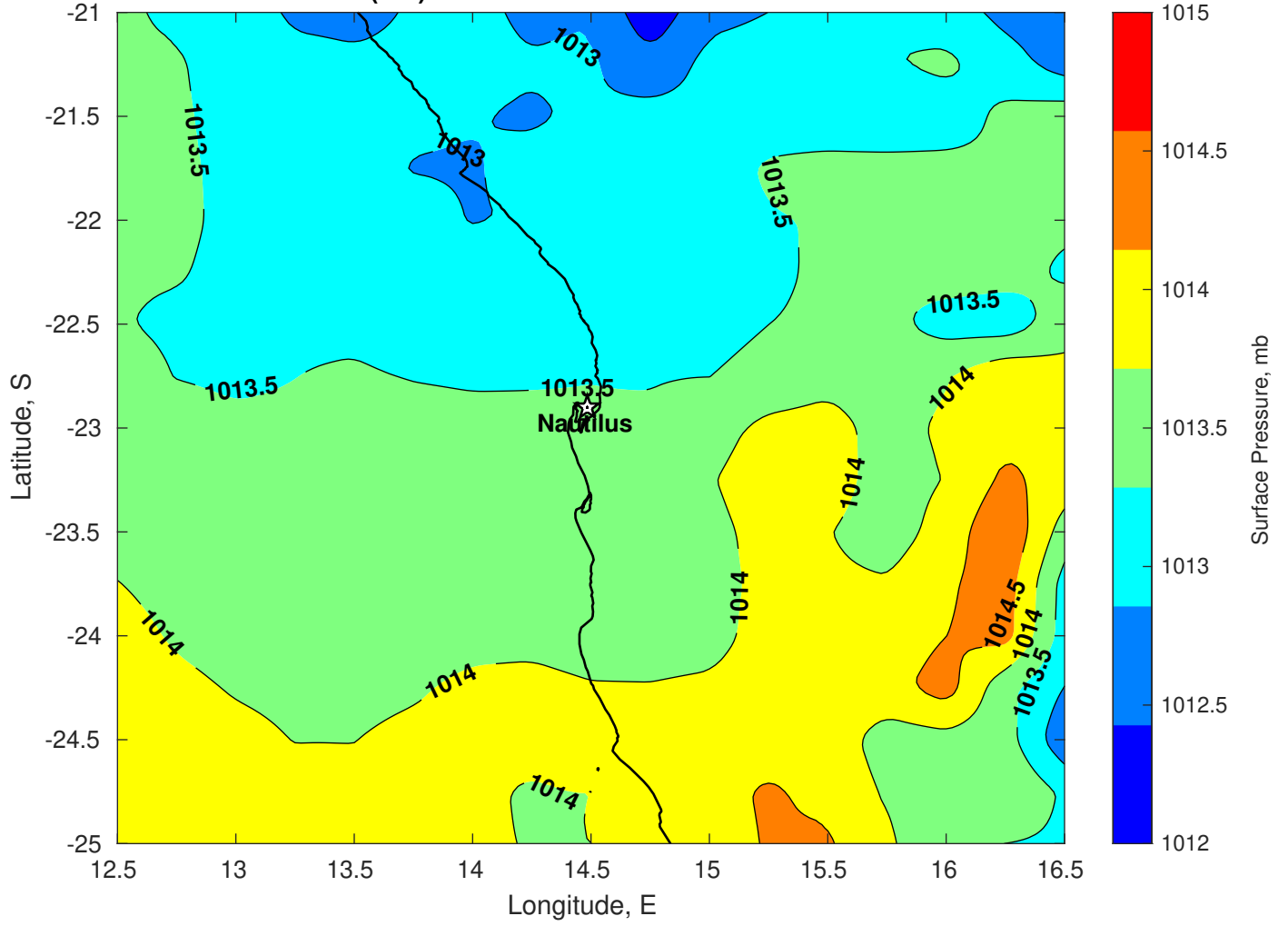
Surface Pressure (mb) for Nautilus at 23-Jan-2025 00:00:00
