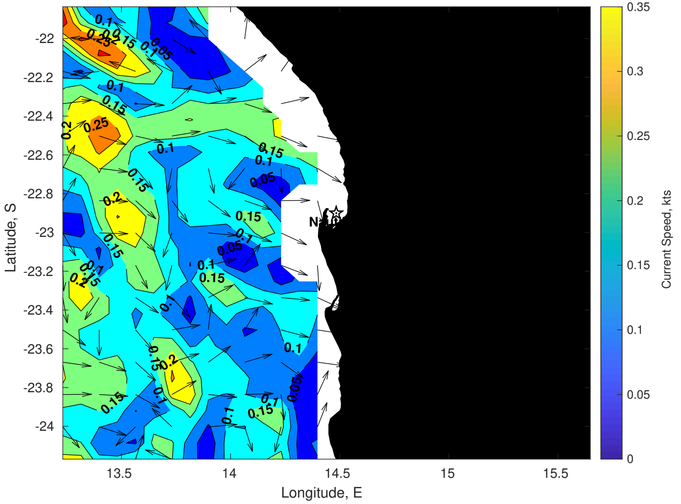
Surface Currents for Nautilus at 22-Jan-2025 00:00:00
