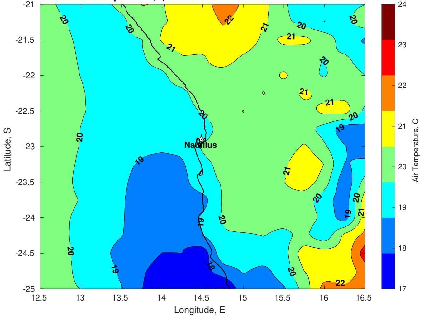
Air Temperature (C) for Nautilus at 23-Jan-2025
