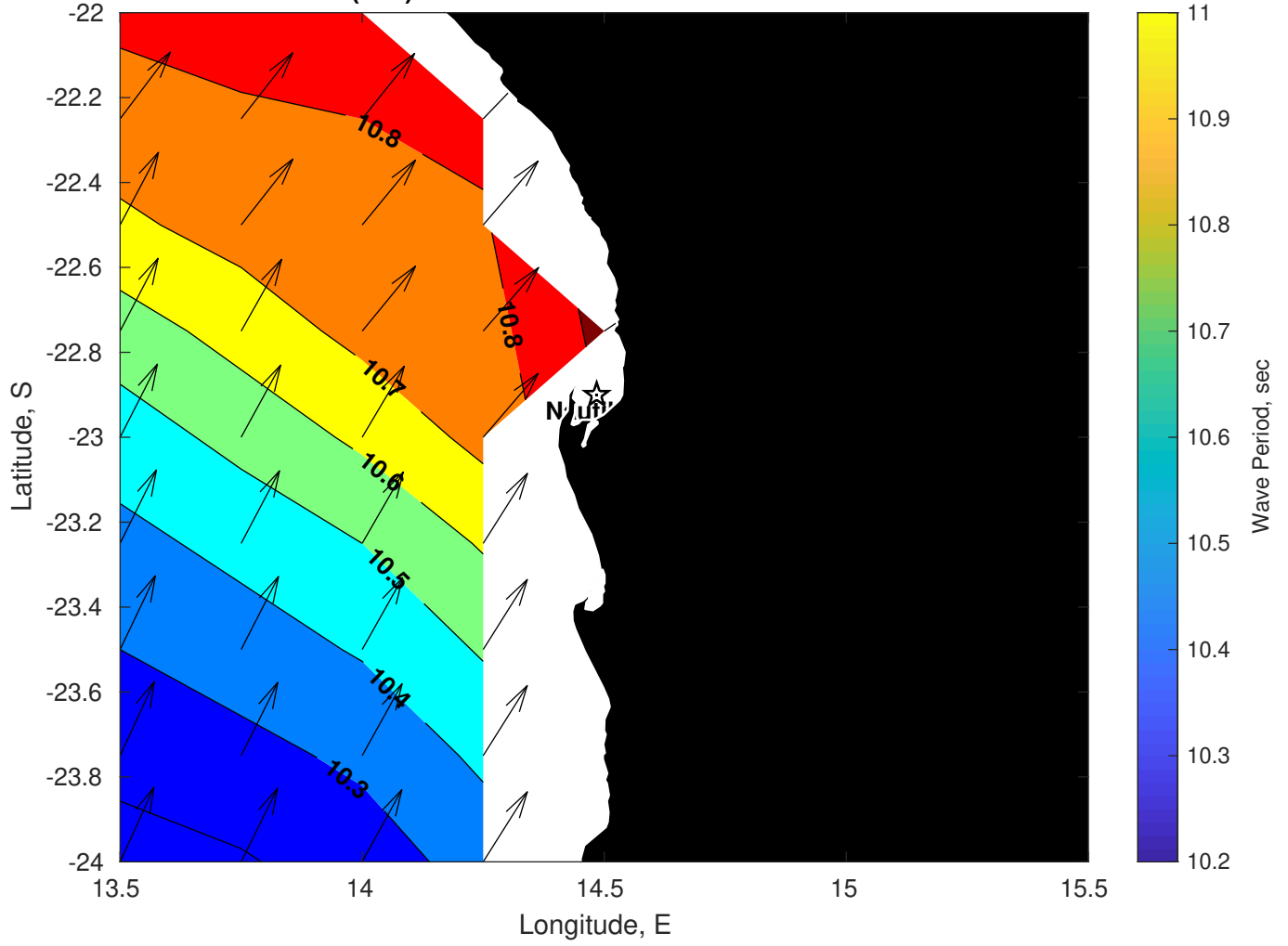
Wave Period (sec) for Nautilus at 23-Jan-2025 09:00:00
