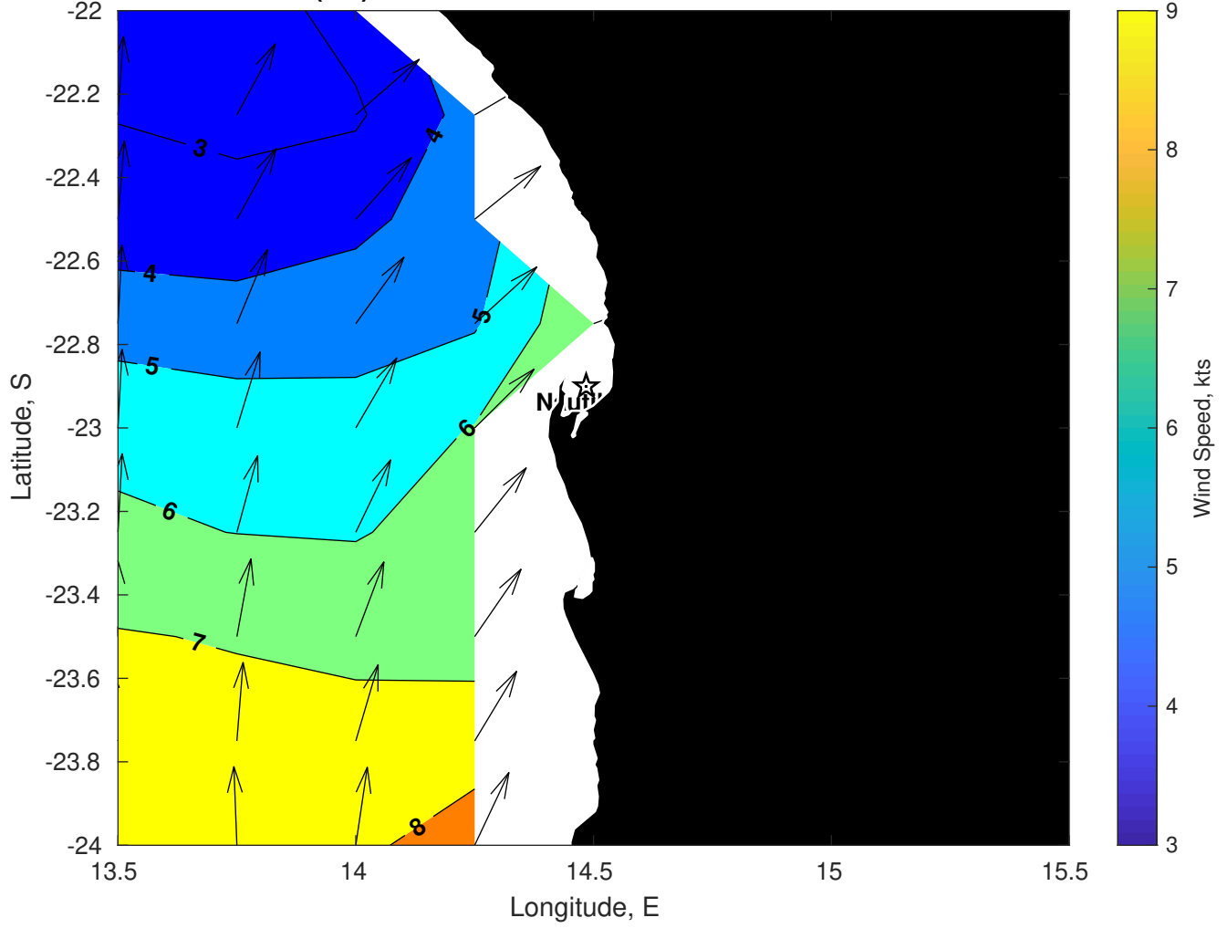
Winds (kts) for Nautilus at 23-Jan-2025 09:00:00
