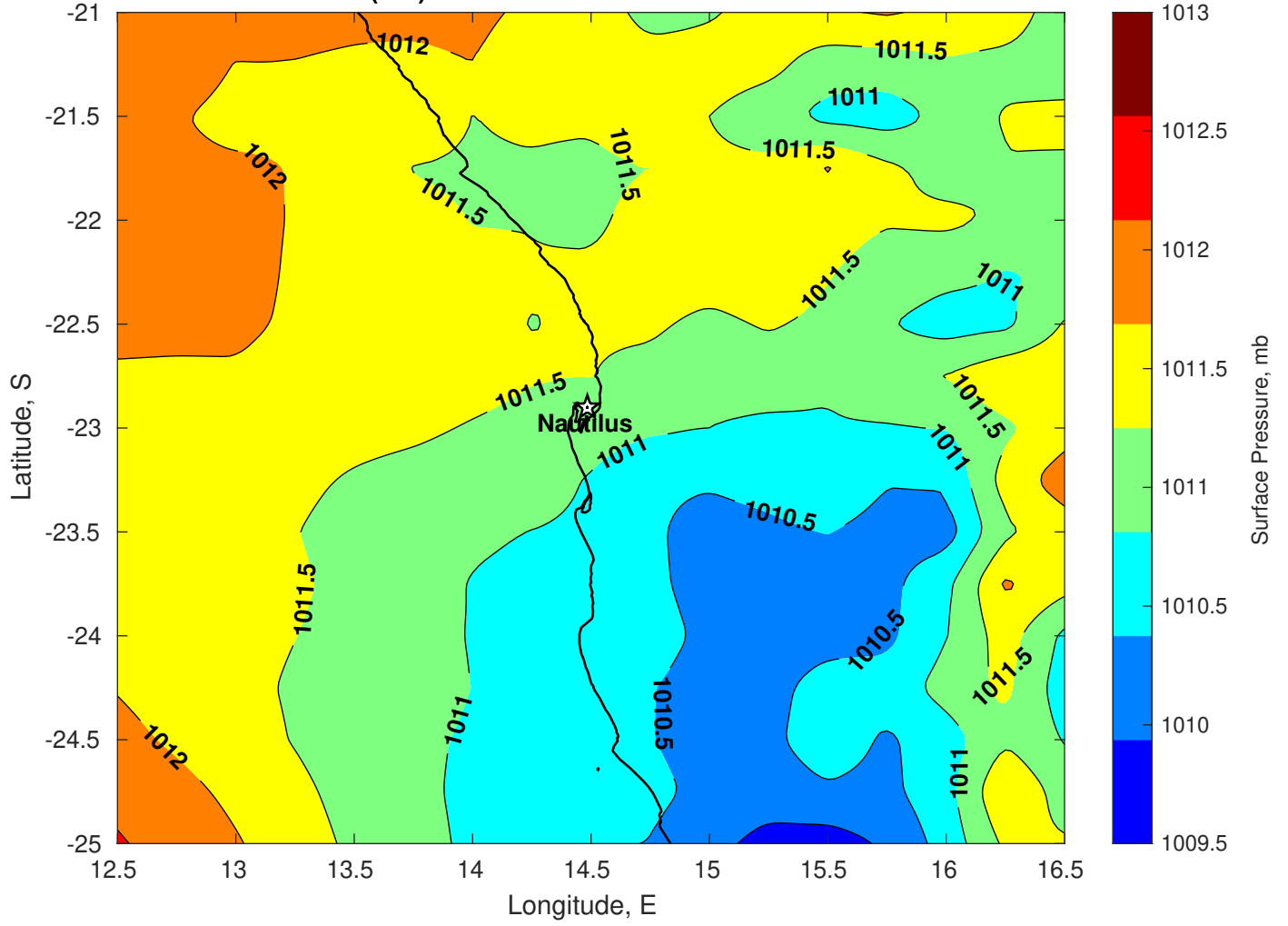
Surface Pressure (mb) for Nautilus at 24-Jan-2025 00:00:00
