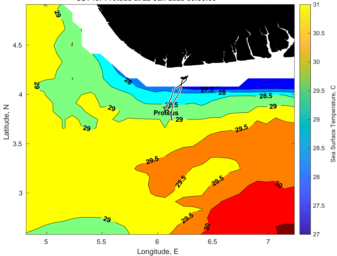
SST for Proteus at 22-Jan-2025 00:00:00
