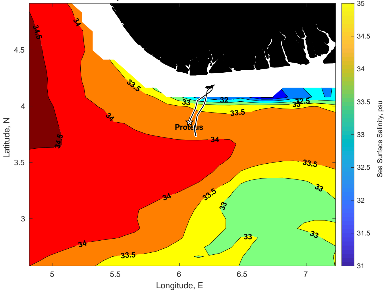
Surface Salinity for Proteus at 22-Jan-2025 00:00:00
