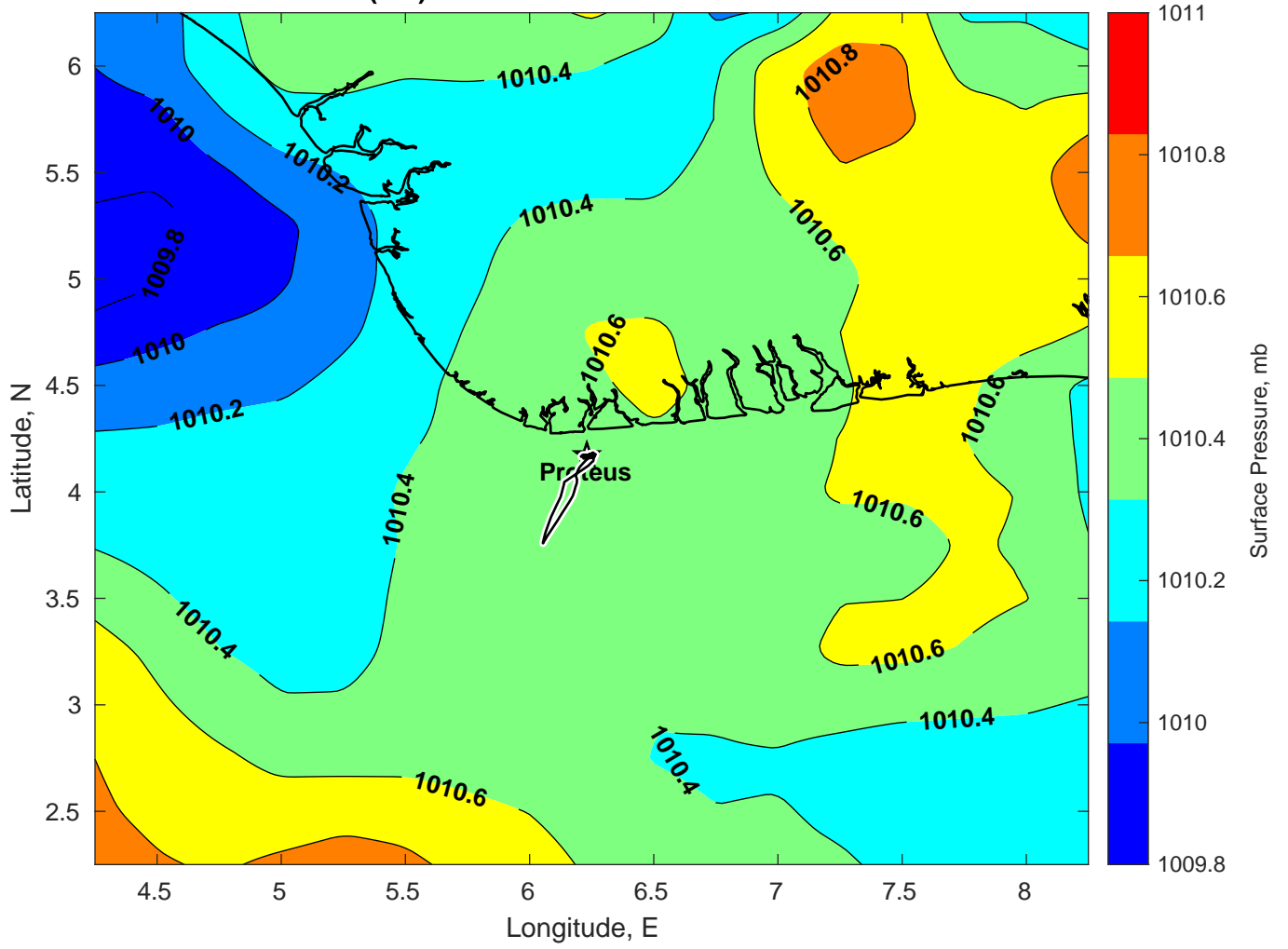
Surface Pressure (mb) for Proteus at 24-Jan-2025 00:00:00
