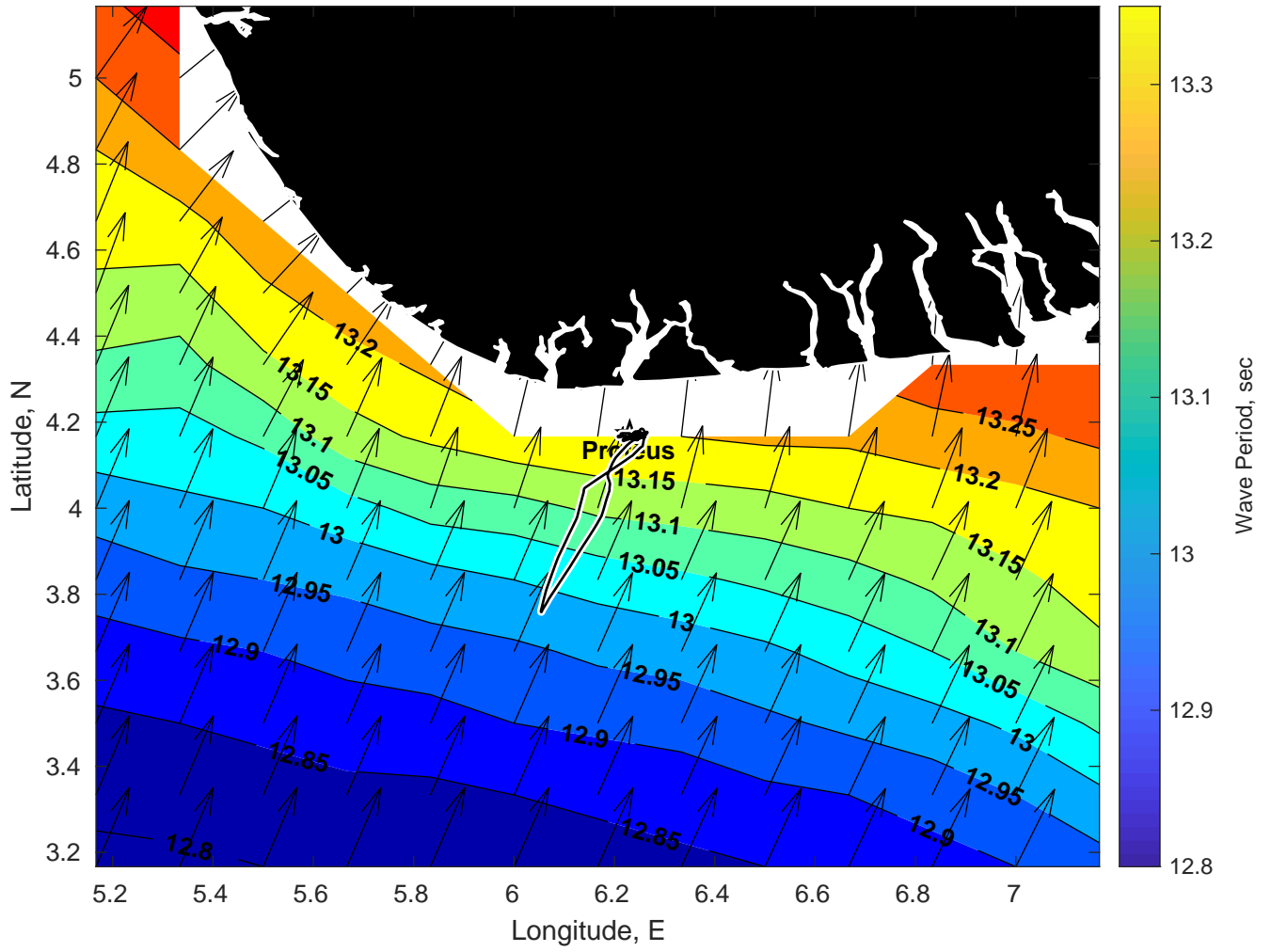
Wave Period (sec) for Proteus at 23-Jan-2025 09:00:00
