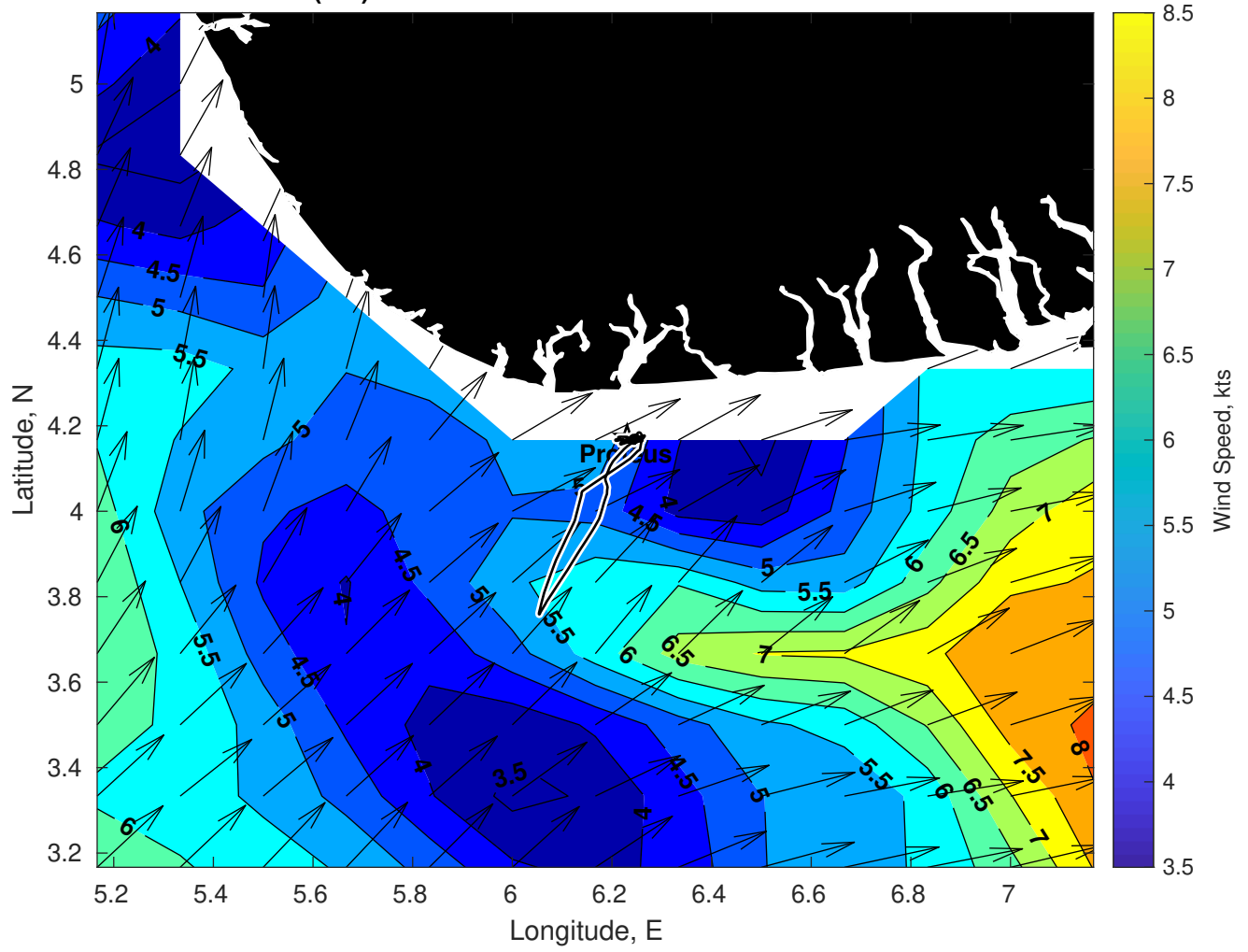
Winds (kts) for Proteus at 23-Jan-2025 09:00:00
