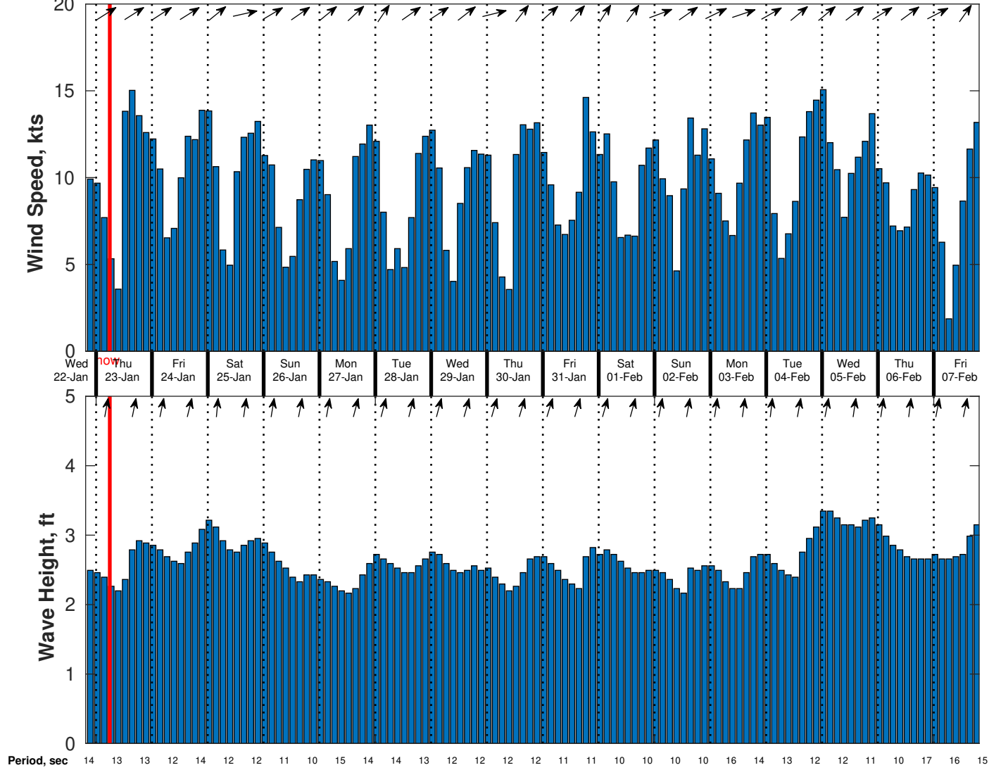
Wind & Wave Forecast for Proteus from 22-Jan-2025 20:00:00 to 07-Feb-2025 20:00:00
