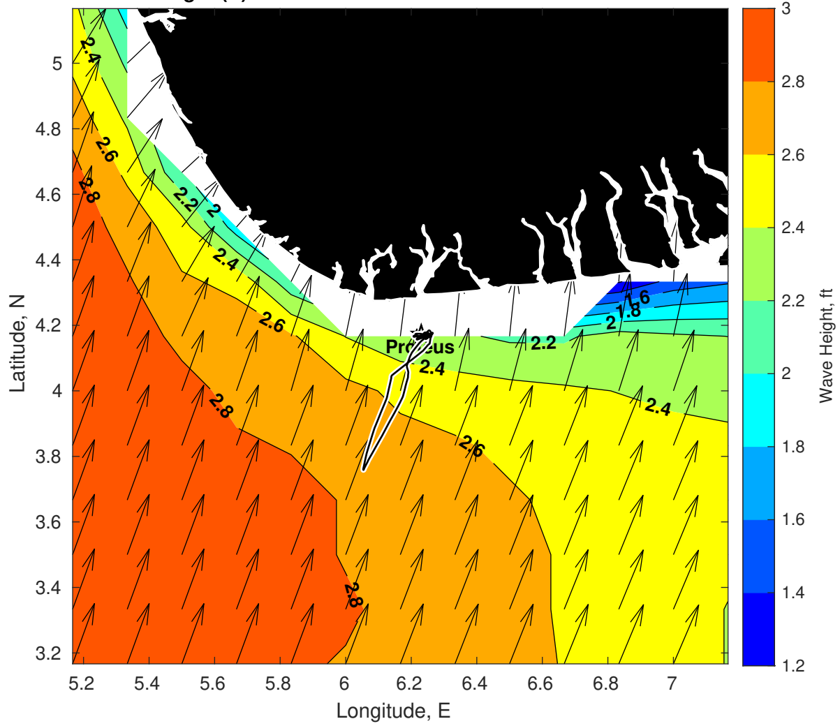
Wave Height (ft) for Proteus at 23-Jan-2025 09:00:00
