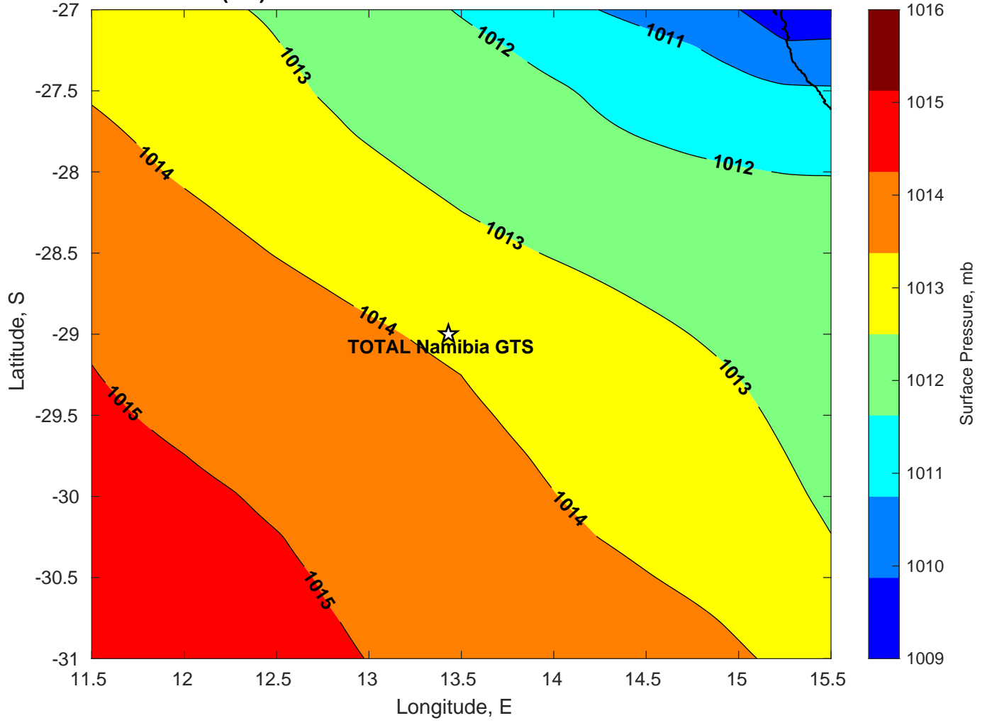
Surface Pressure (mb) for TOTAL Namibia GTS at 25-Jan-2025 00:00:00
