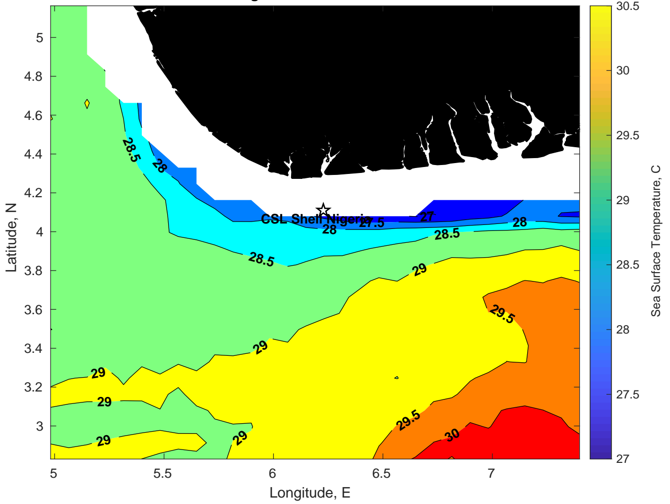
SST for CSL Shell Nigeria at 23-Jan-2025 00:00:00
