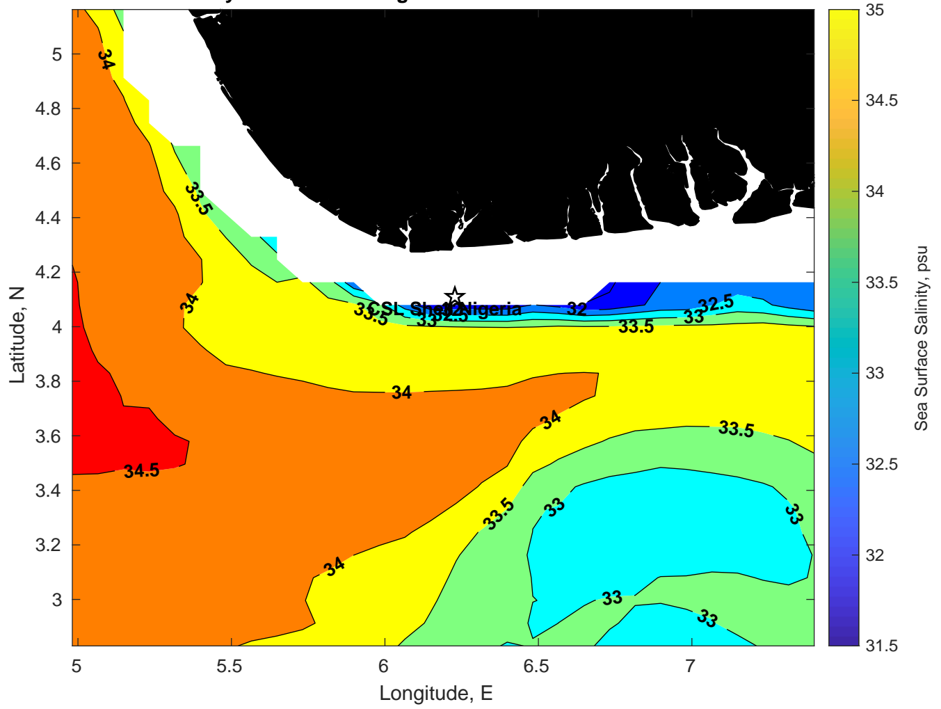
Surface Salinity for CSL Shell Nigeria at 23-Jan-2025 00:00:00
