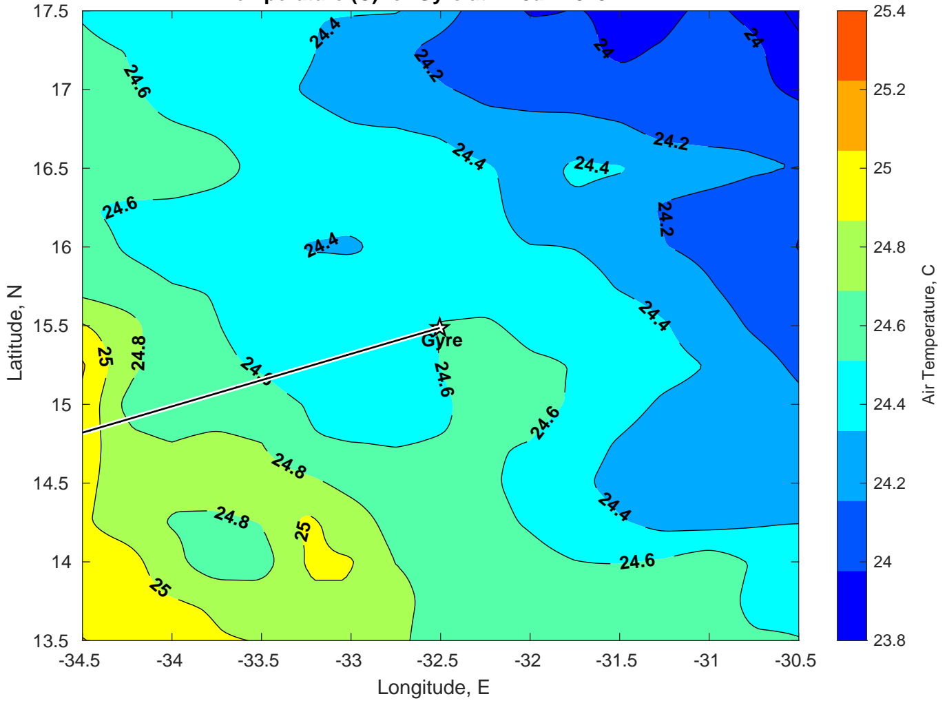
Air Temperature (C) for Gyre at 24-Jan-2025
