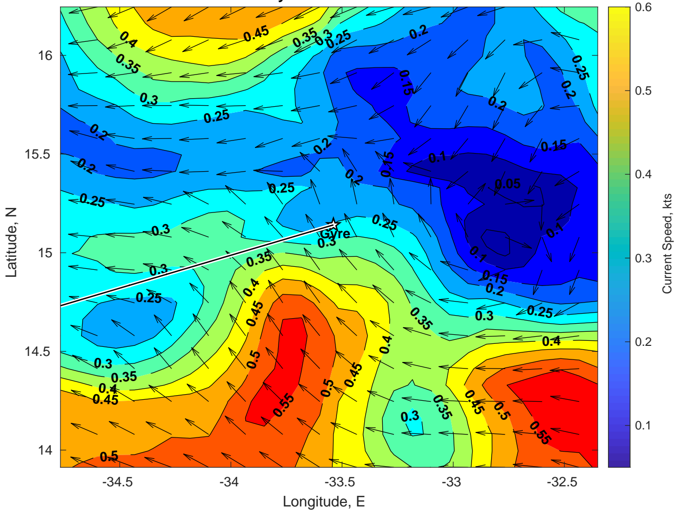
Surface Currents for Gyre at 23-Jan-2025 00:00:00
