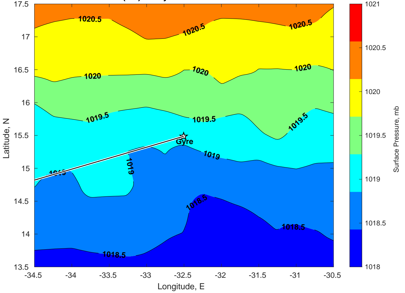
Surface Pressure (mb) for Gyre at 26-Jan-2025 00:00:00
