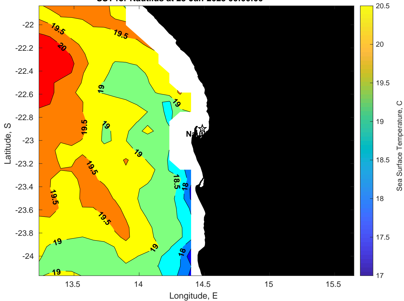
SST for Nautilus at 23-Jan-2025 00:00:00
