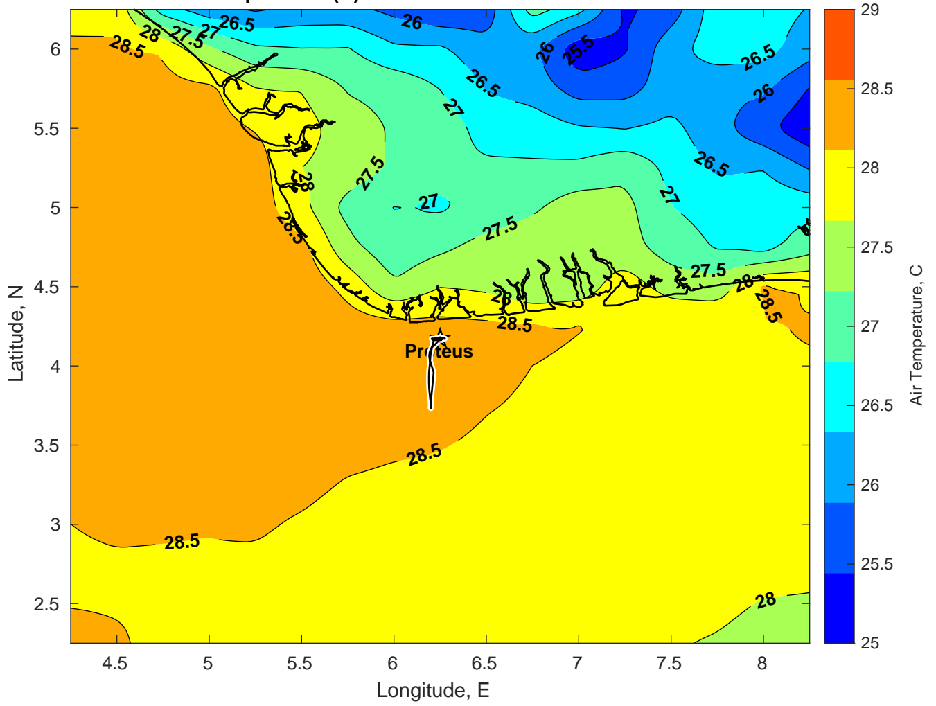
Air Temperature (C) for Proteus at 24-Jan-2025
