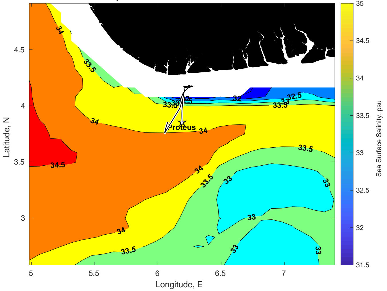
Surface Salinity for Proteus at 23-Jan-2025 00:00:00
