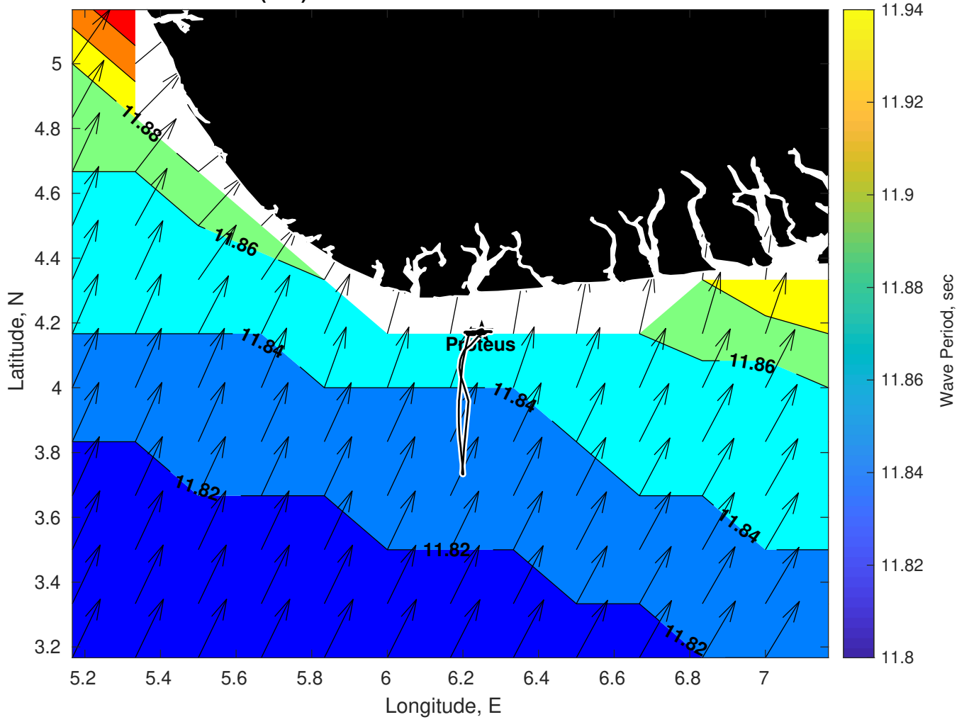
Wave Period (sec) for Proteus at 24-Jan-2025 09:00:00
