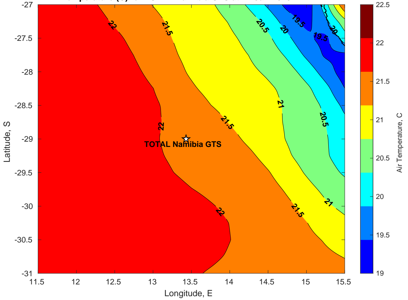
Air Temperature (C) for TOTAL Namibia GTS at 24-Jan-2025
