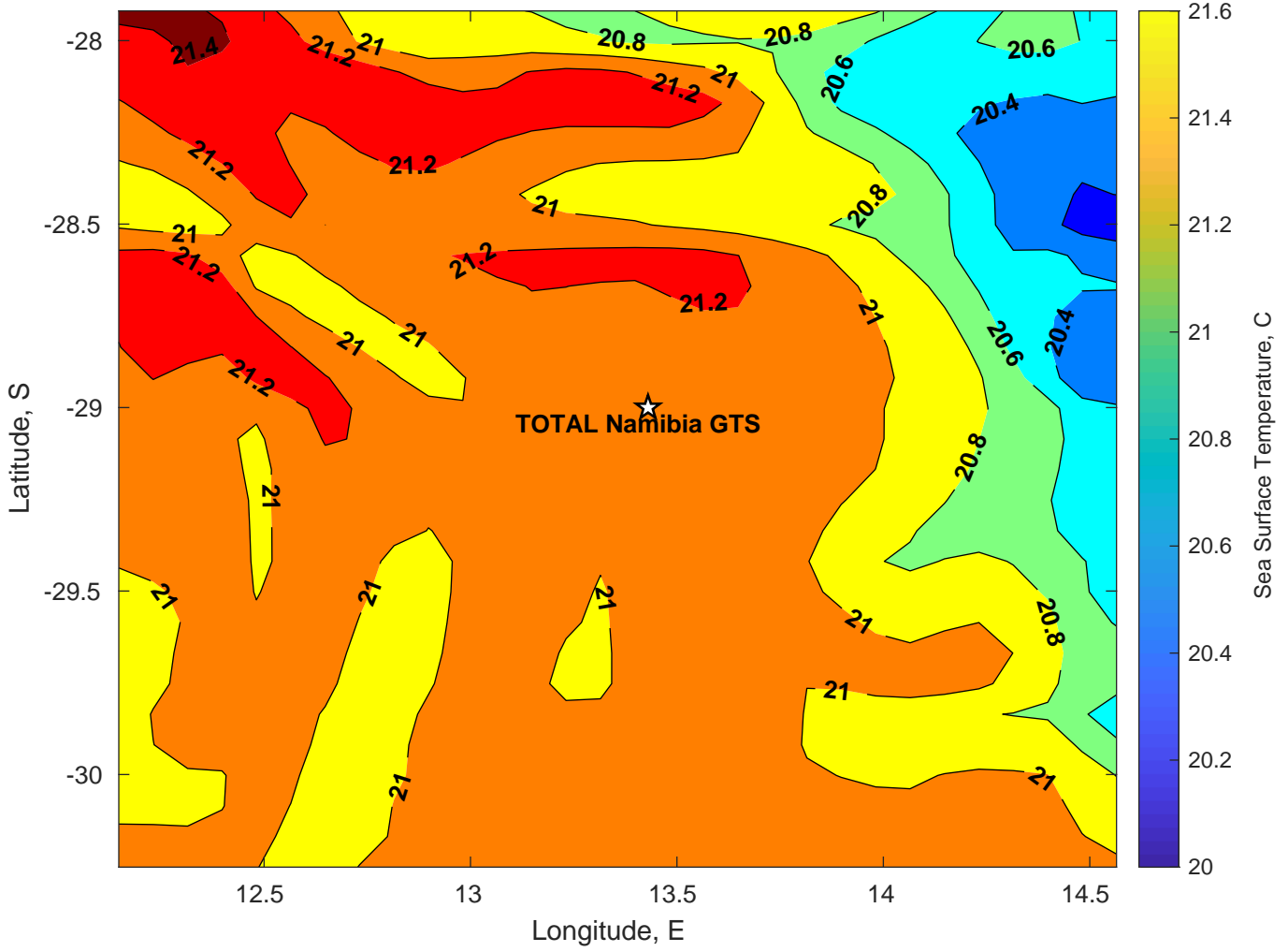
SST for TOTAL Namibia GTS at 23-Jan-2025 00:00:00
