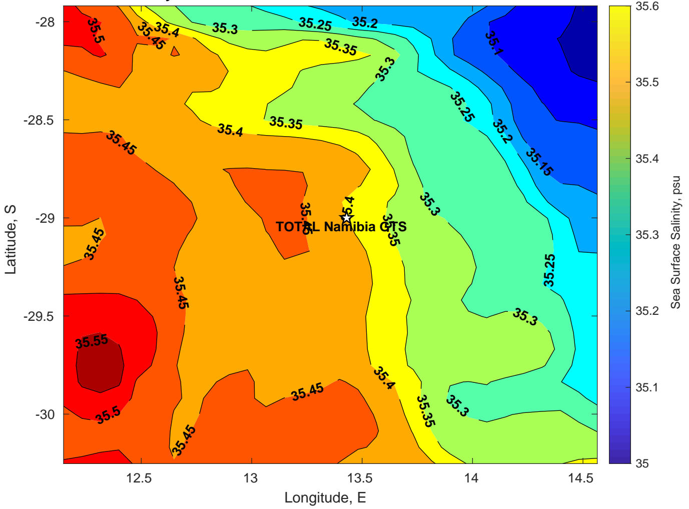
Surface Salinity for TOTAL Namibia GTS at 23-Jan-2025 00:00:00
