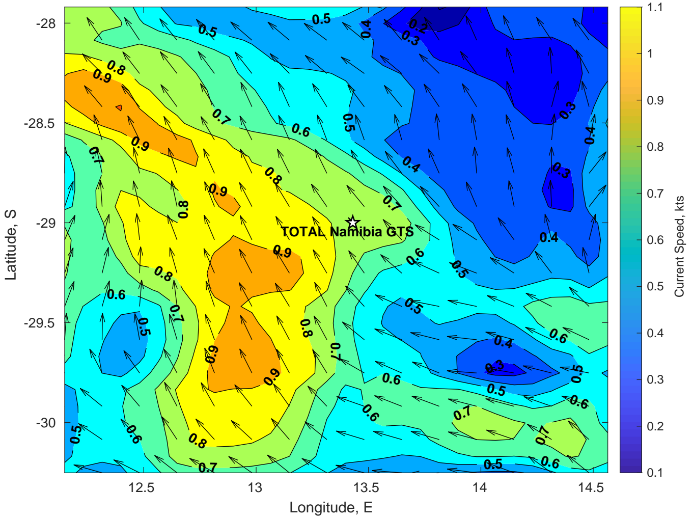
Surface Currents for TOTAL Namibia GTS at 23-Jan-2025 00:00:00
