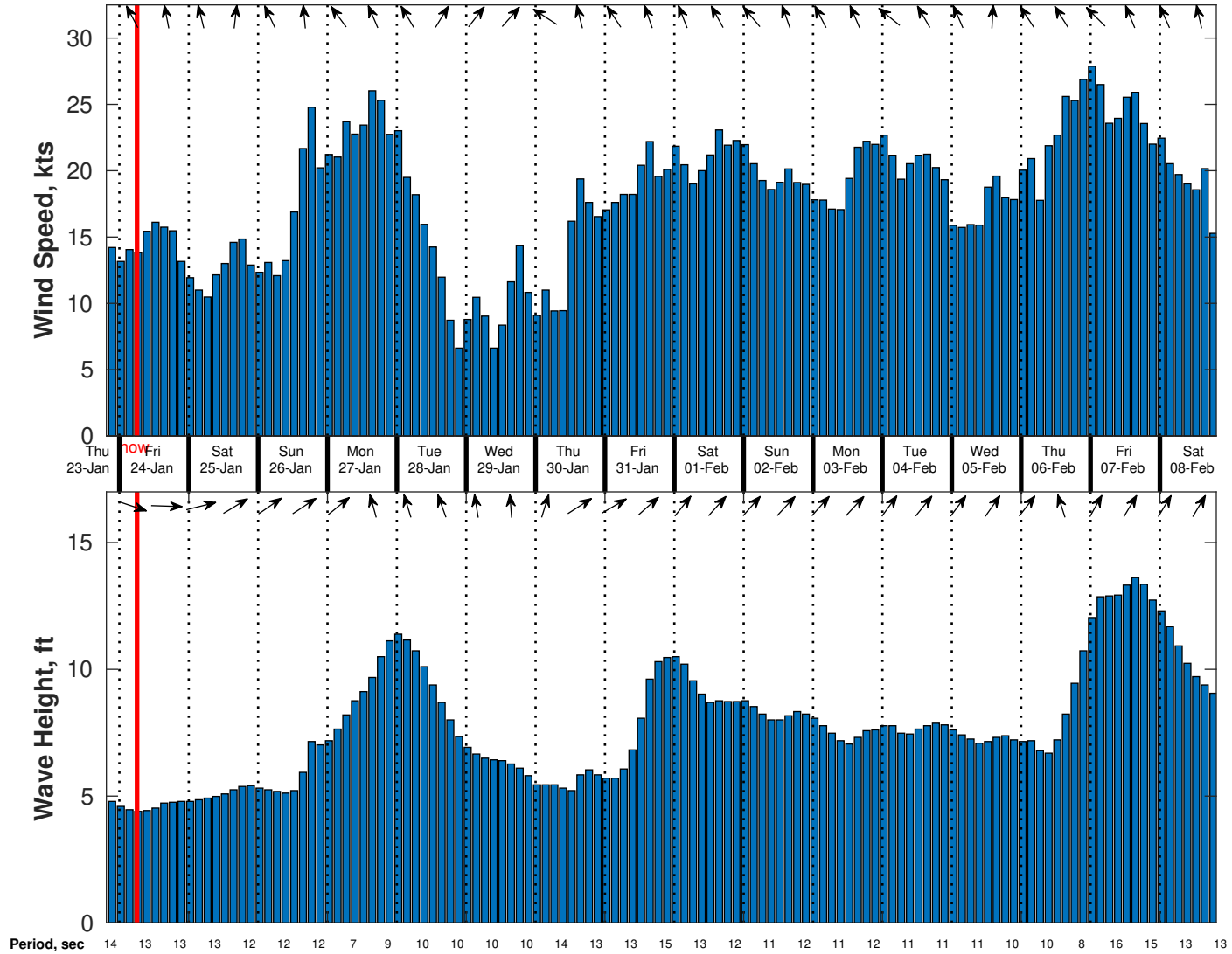
Wind & Wave Forecast for TOTAL Namibia GTS from 23-Jan-2025 20:00:00 to 08-Feb-2025 20:00:00
