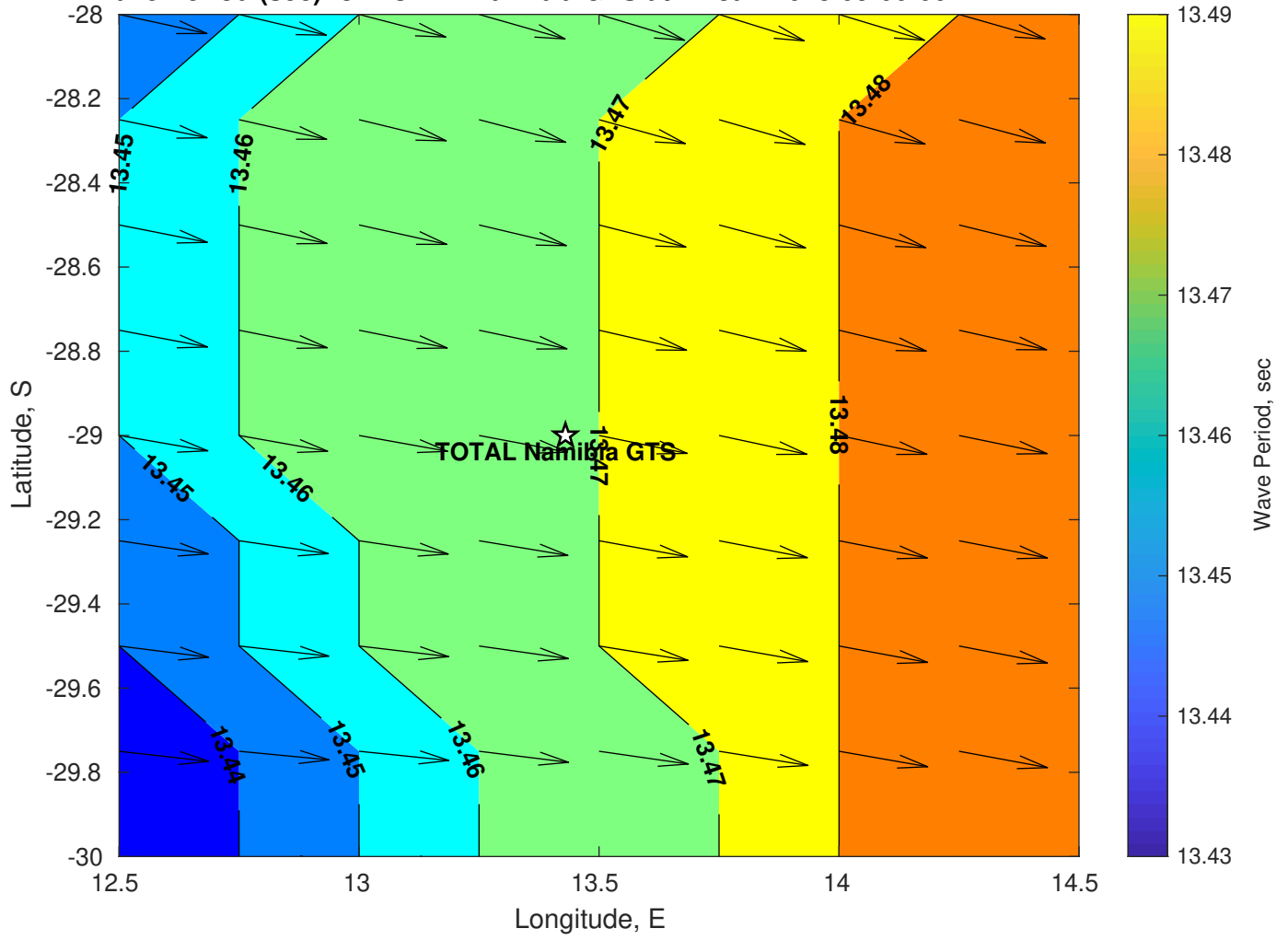
Wave Period (sec) for TOTAL Namibia GTS at 24-Jan-2025 09:00:00
