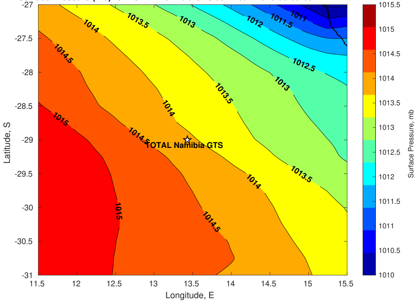
Surface Pressure (mb) for TOTAL Namibia GTS at 24-Jan-2025 00:00:00
