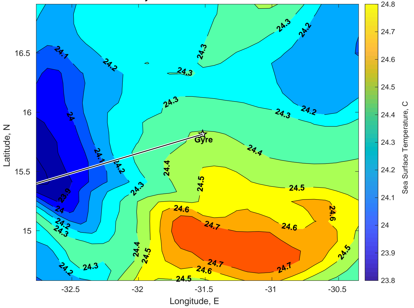
SST for Gyre at 24-Jan-2025 00:00:00
