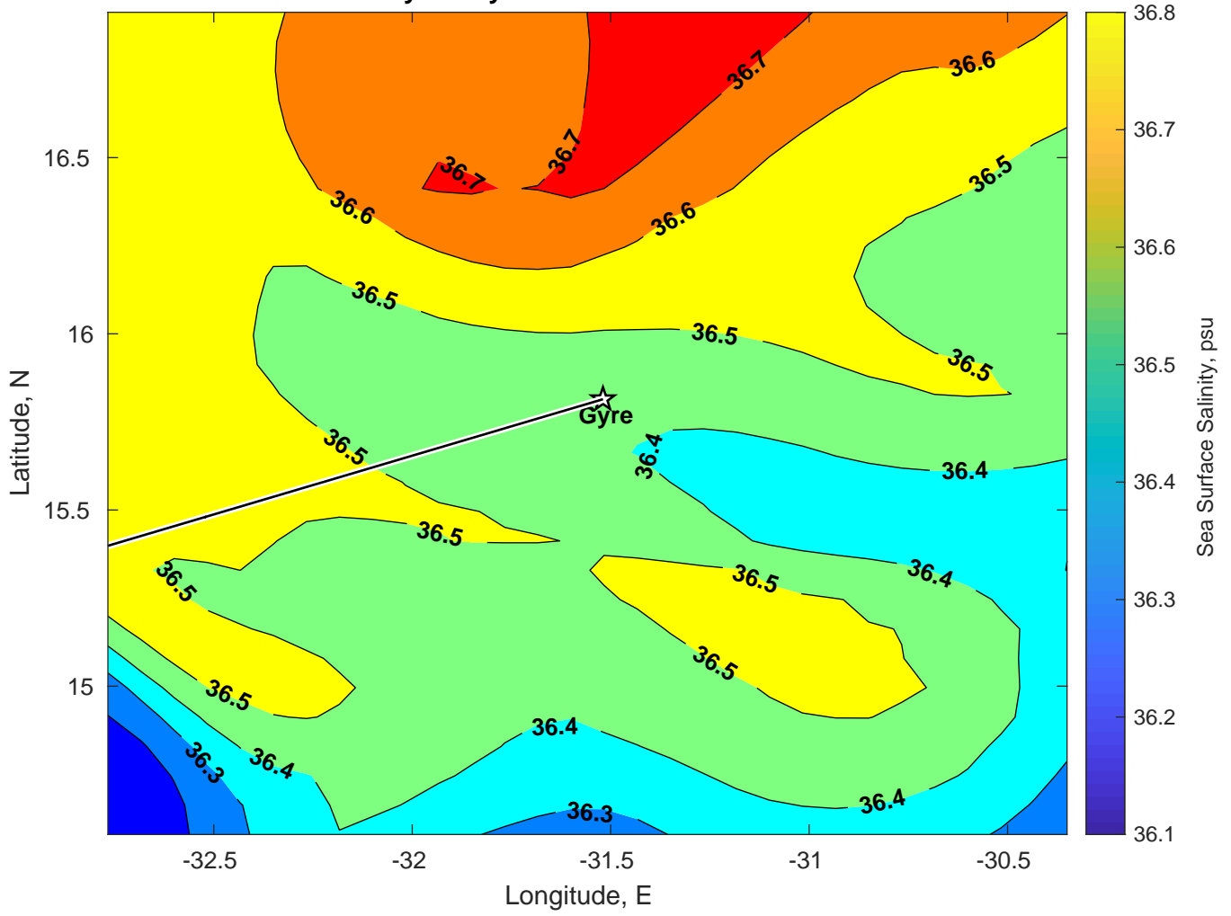
Surface Salinity for Gyre at 24-Jan-2025 00:00:00
