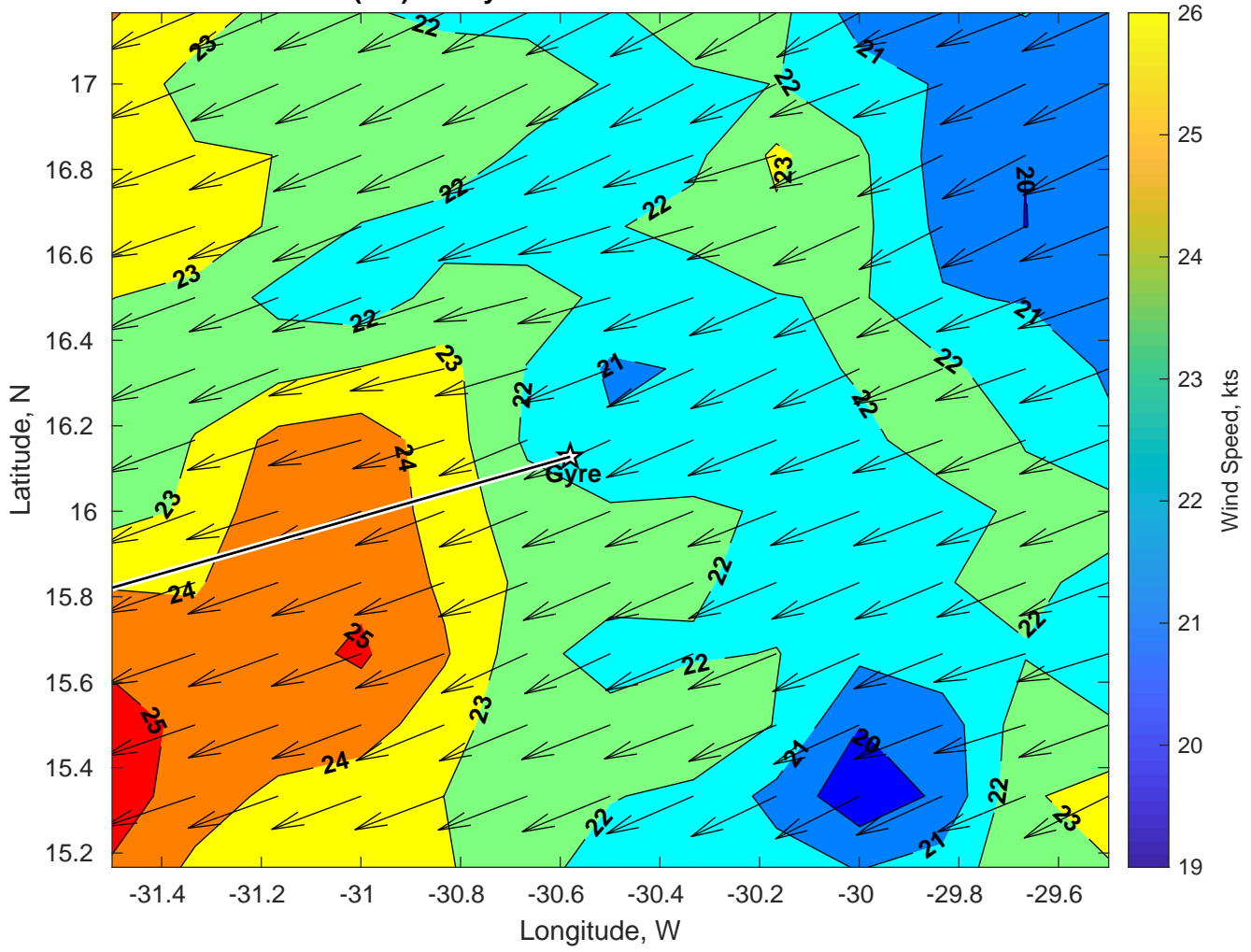
Winds (kts) for Gyre at 25-Jan-2025 09:00:00
