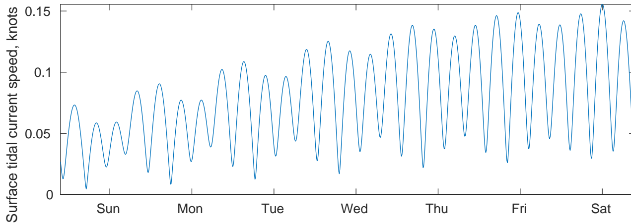
Tidal Currents and Heights for Gyre at 20250125
