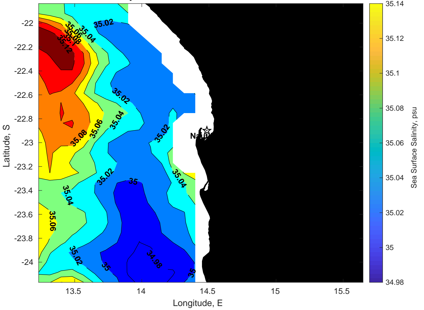
Surface Salinity for Nautilus at 24-Jan-2025 00:00:00
