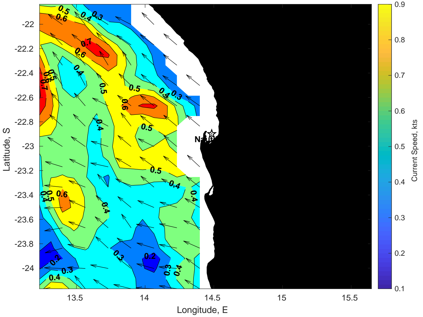
Surface Currents for Nautilus at 24-Jan-2025 00:00:00
