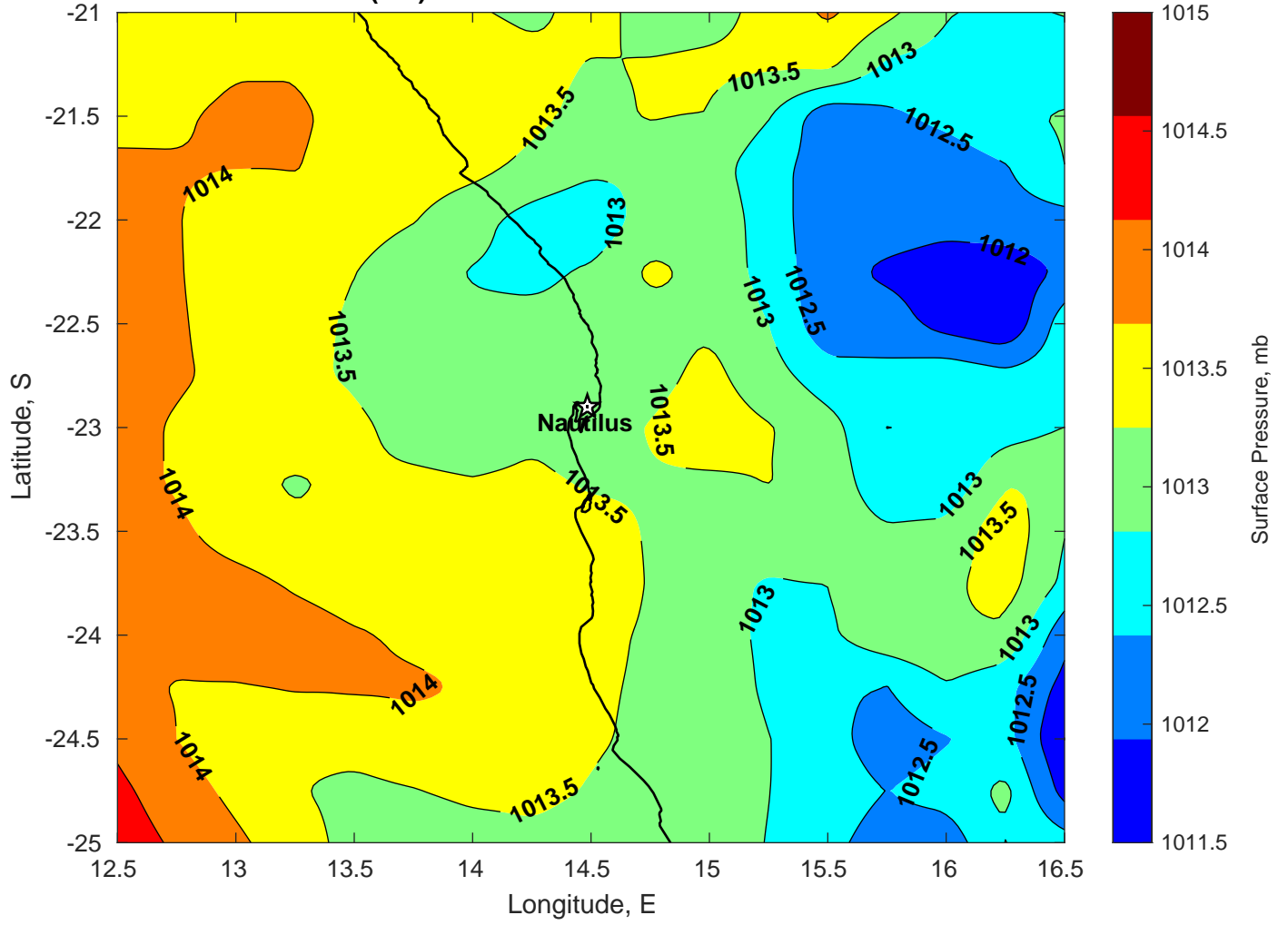
Surface Pressure (mb) for Nautilus at 26-Jan-2025 00:00:00
