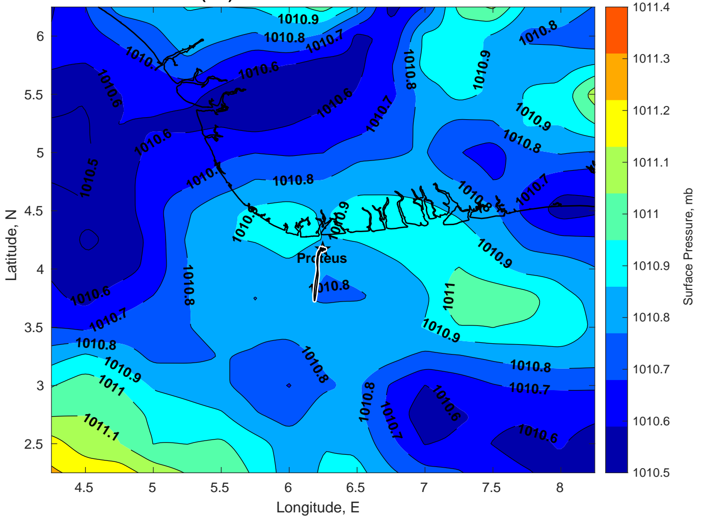
Surface Pressure (mb) for Proteus at 25-Jan-2025 00:00:00
