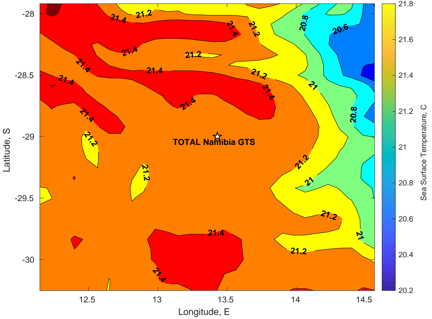
SST for TOTAL Namibia GTS at 24-Jan-2025 00:00:00
