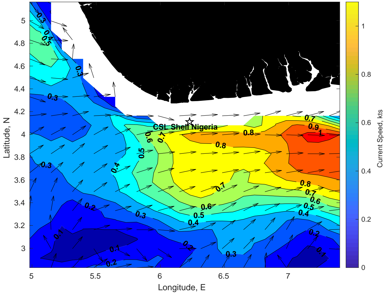
Surface Currents for CSL Shell Nigeria at 25-Jan-2025 00:00:00
