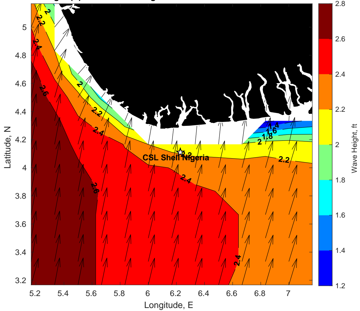
Wave Height (ft) for CSL Shell Nigeria at 26-Jan-2025 09:00:00
